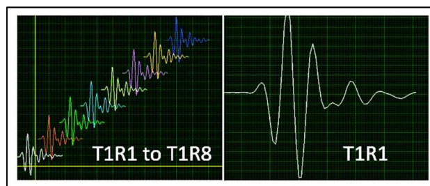
Fig. 10. PAUT normal wave results
