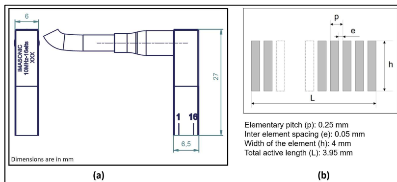
Fig. 3. (a) Mechanical drawing and (b) elements layout of the Imasonic Small-footprint array [image produced by Imasonic]
