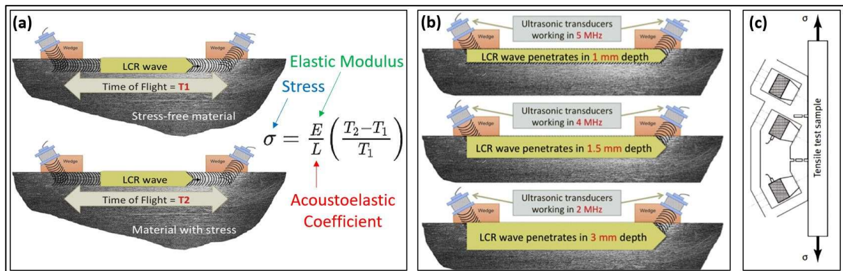
Fig. 1. (a) Principles of the ultrasonic stress measurement [13], (b) the possibility of through-thickness stress measurement [13] and (c) tensile test for measurement of the acoustoelastic coefficient [9]
