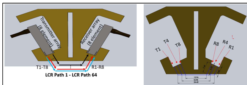
Fig. 7. LCR Path distance in the PAUT-LCR system
