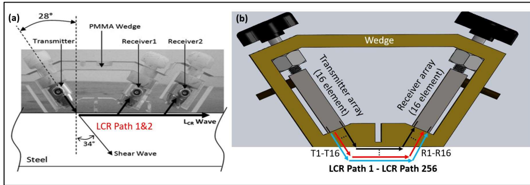
Fig. 2. (a) Traditional ultrasonic LCR stress measurement [9] and (b) PAUT-LCR stress measurement approach developed in this paper
