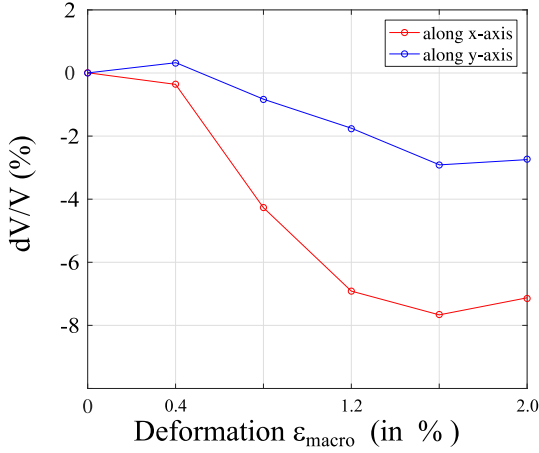
Figure 16. dV_x/V_x and dV_y/V_y divided by their respective initial values as functions of the macroscopic deformation. The velocities are calculated with the time of flight of the summed signals along the reception wall for a low-frequency pulse (150 kHz).
