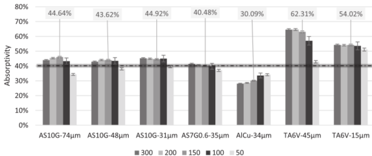
Fig. 9. Average absorptance measurements for several powders and material for 0.2 mm - powder bed layer thickness from 50 to 300 µm - highlighted values: mean - line: absorptivity of the substrate.
