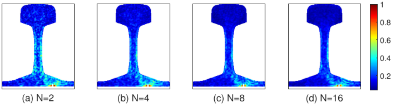
Fig. 11. Topological images of the rail section presenting a longitudinal vertical crack. The defect is represented by a white line. Each image is computed considering 2, 4, 8 and 16 transducers. The polarization is in the rail plane. The acquisition duration is 300 \mu s.
