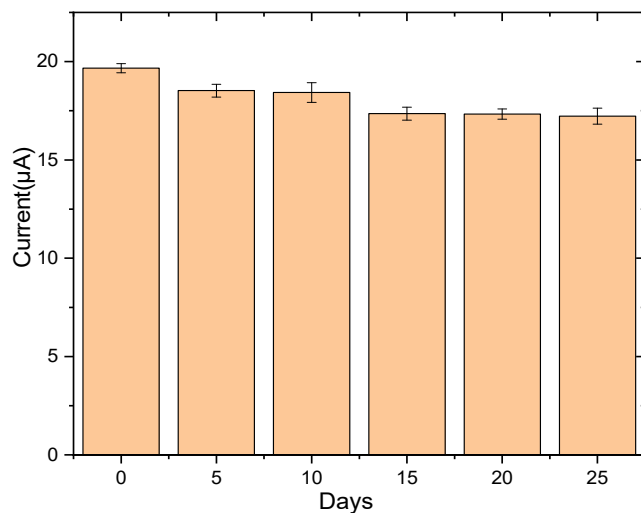
Figure 13. Responses obtained from the MIP-GCE/OPPy/CuNPs sensor in \text{H}_2\text{SO}_4 solution containing 10^{-6} mol \text{L}^{-1} of SDZ.
