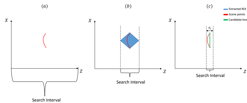
Figure 9. An illustrative figure of the three experimental configurations: (a) the depth value is searched over the whole space; (b) regions of interest are used to delimit the search interval; (c) the regions of interest are refined, and a fixed size interval of size N_z + 1 centered on the predicted optimal representation line is used as the search interval.
