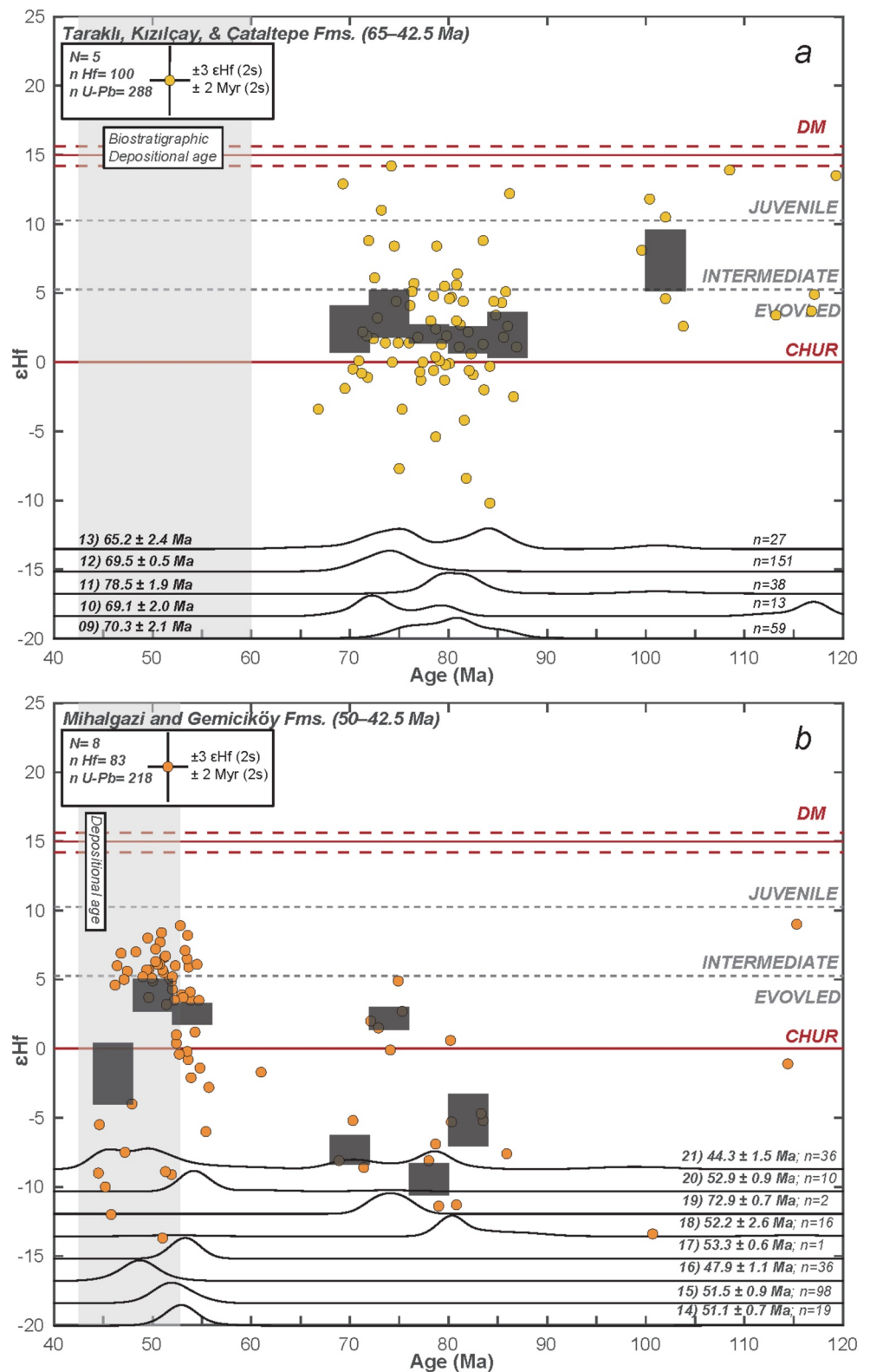
Figure 5. Zircon U-Pb versus \epsilon_{\text{Hf}} data from (a) the 65–42.5 Ma Taraklı, Kızılcay, and Çataltepe Formations which overlie the Yenipazar Formation and (b) the stratigraphically highest 50–42.5 Ma Mihalgazi and Gemicköy Formations. Zircon maximum depositional ages are next to sample numbers. Gray columns reflect the units depositional age based on biostratigraphy. All “n” and “n U-Pb” reflect ages between 120 and 40 Ma. Opaque boxes display the 4 Myr binned standard error. CHUR (chondritic uniform reservoir), DM (depleted mantle).
