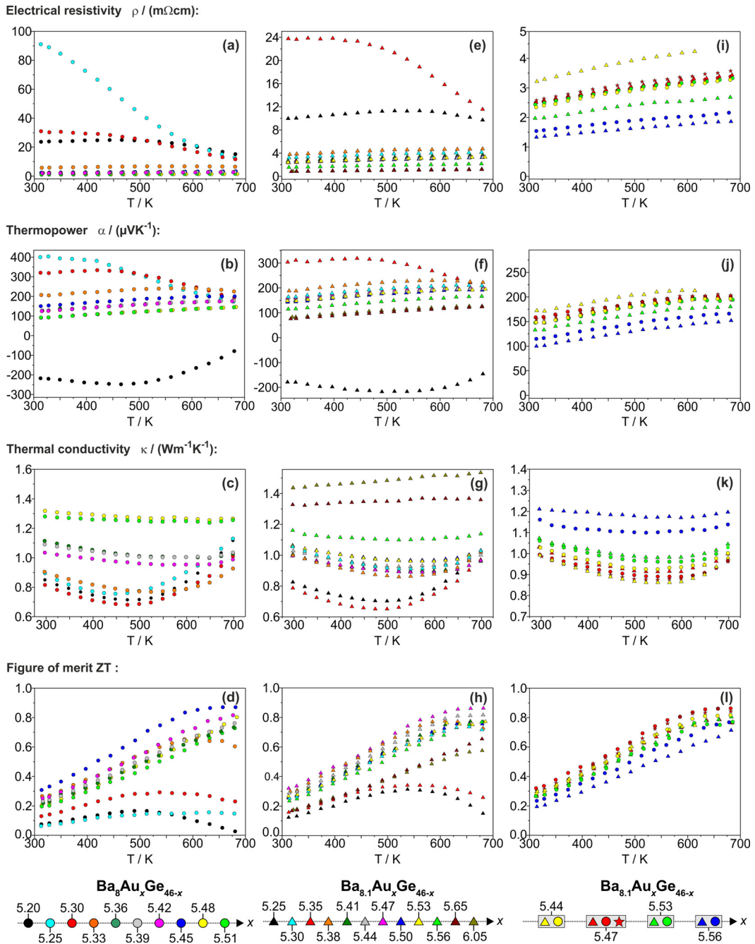
FIG. 3. Temperature dependence of thermoelectric properties between 300 and 700 K. Electrical resistivity \rho , thermopower \alpha , thermal conductivity \kappa , and the dimensionless thermoelectric figure of merit ZT of samples with nominal compositions \text{Ba}_8\text{Au}_x\text{Ge}_{46-x} (a)–(d) and \text{Ba}_{8.1}\text{Au}_x\text{Ge}_{46-x} (e)–(h). Reproducibility of the thermoelectric properties for different batches with the same composition in the series \text{Ba}_{8.1}\text{Au}_x\text{Ge}_{46-x} (i)–(l).
