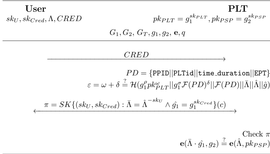
Figure 9: Verify algorithm.
