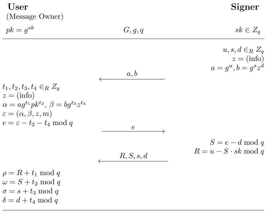
Figure 6: WI-Schnorr partially blind signature.
