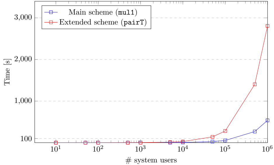
Figure 11: Time complexity of Revoke algorithm.
