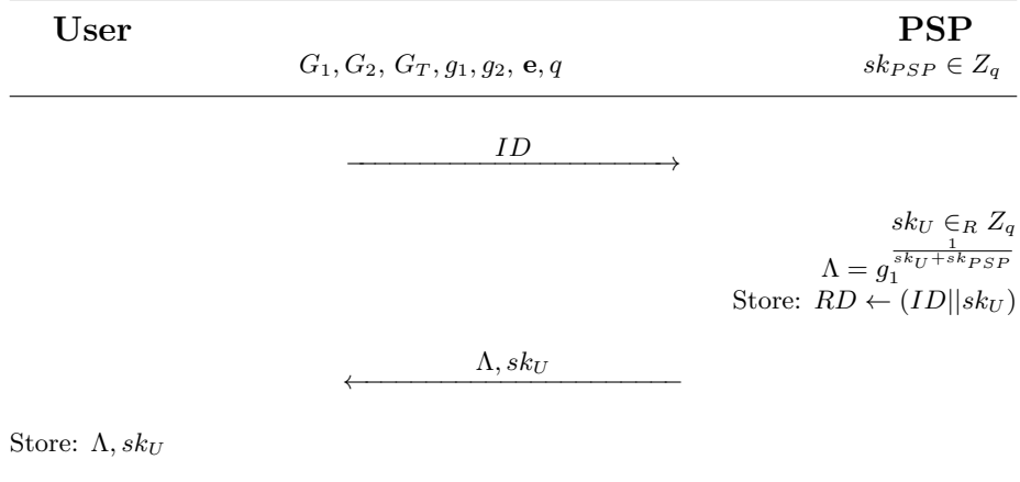
Figure 7: Register algorithm.
