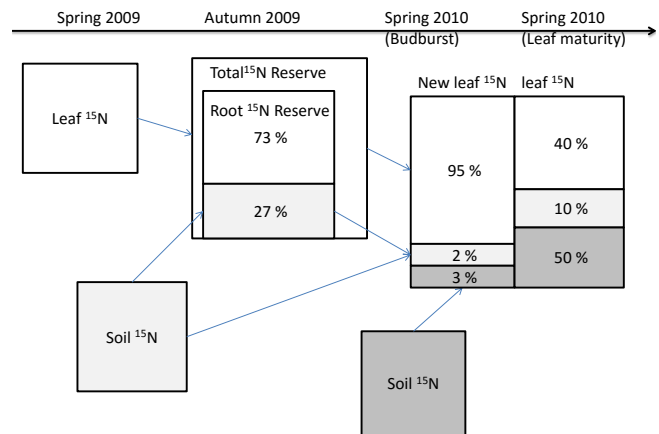
Figure 4. Conceptual scheme representing percentage contributions of ^{15}\text{N} (Eq. 2) from each labelling campaign ( L_1 : white, L_2 : light grey, L_3 : dark grey) in roots in the autumn and in new leaves in the season following the first labelling campaign.
