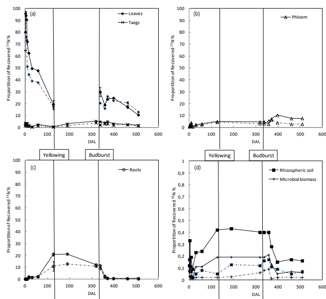
Figure 1. Partitioning of recovered ^{15}\text{N} (PRN%) from the sampled compartments following the first labelling campaign, i.e. from 27 May 2009 to 20 October 2010. (a) Leaves \blacklozenge and twigs \times , (b) phloem \triangle , (c) fine roots \circ , (d) rhizospheric soil \blacksquare and microbial biomass + (for those compartments the Y axis was adjusted to 1). DAL: days after labelling. The two lines, continuous and dotted, correspond to tree 1 and tree 2. Vertical bars indicate standard errors.
