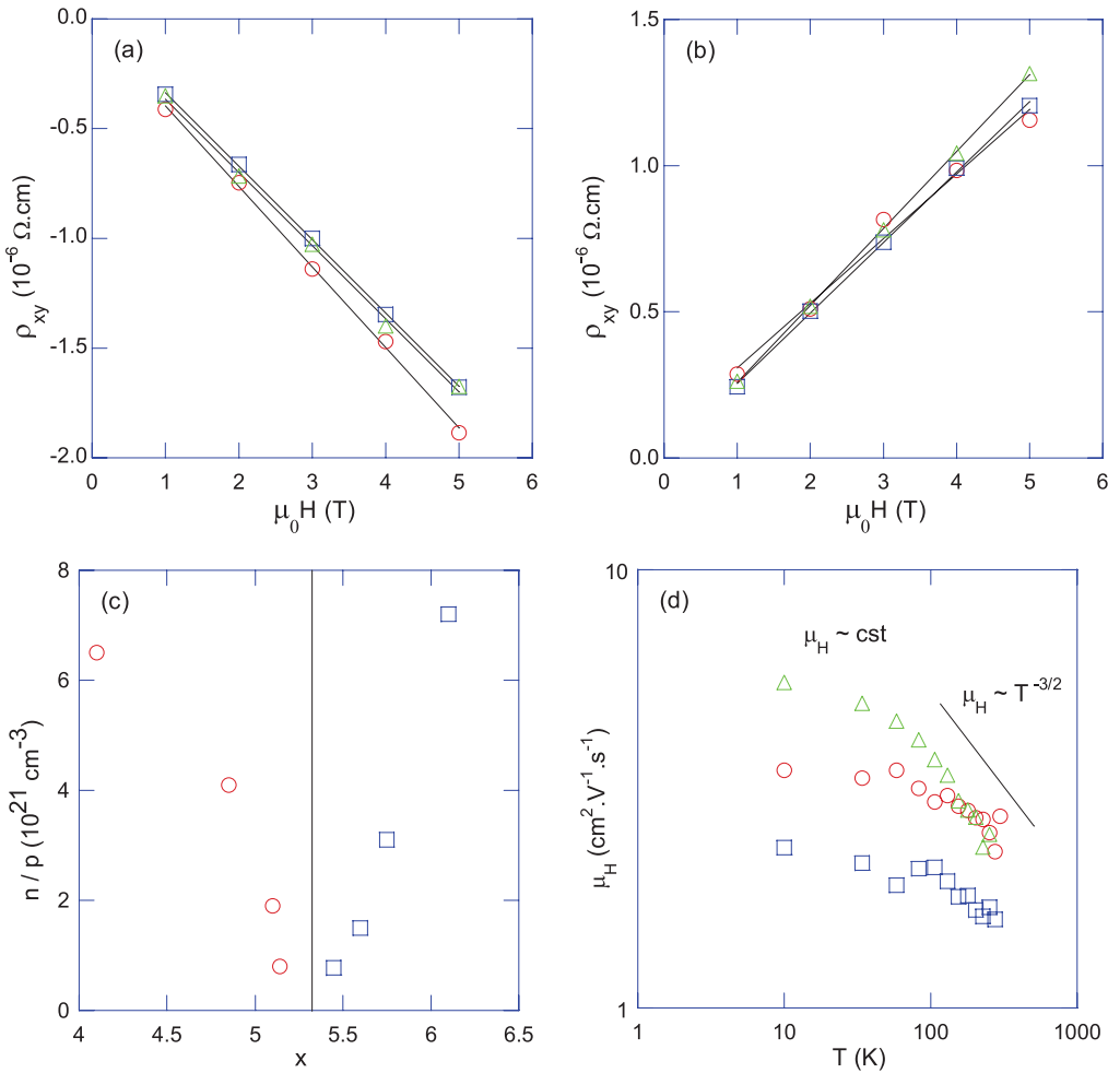
FIG. 8. (Color online) Transverse Hall resistivity \rho_{xy} as a function of the magnetic field \mu_0 H of \text{Ba}_8\text{Au}_x\text{Si}_{46-x} for (a) x = 5.10 and (b) x = 5.76 measured at (○) 275 K, (□) 105 K, and (△) 35 K and (○) 200 K, (□) 155 K, and (△) 10 K, respectively. The solid black lines stand for the best fit to the data highlighting the linearity of the \rho_{xy}(\mu_0 H) data. (c) (○) Electron and (□) hole concentrations as a function of the Au content. The solid black line delineates the n - and p -type regions according to the Zintl concept ( x = 5.33 ). (d) Temperature dependence of the Hall mobility \mu_H of the x = 5.14, 5.59, and 6.10 samples.
