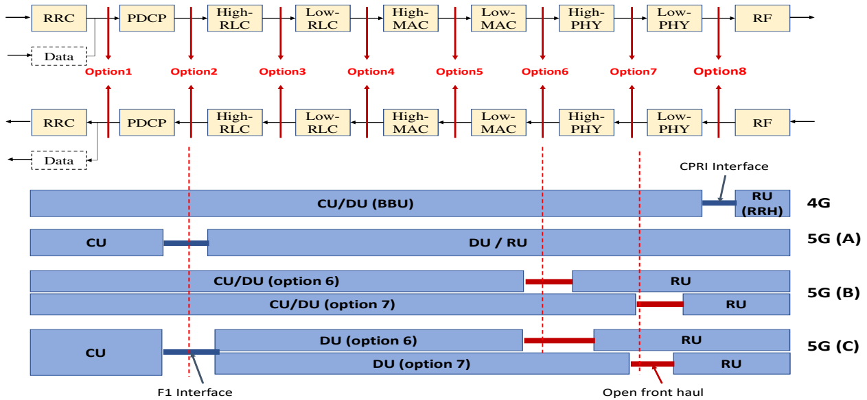
Fig. 6. Splitting options of CU, DU, and RU functions in O-RAN. 5G(A) split of high layer; 5G(B) split of low layer; 5G(C) cascaded split [35].
