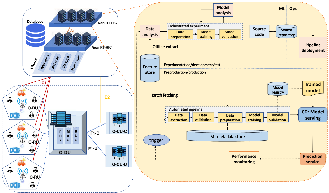
Fig. 11. Automation of ML Process in O-RAN.
