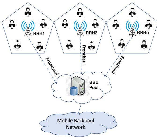
Fig. 3. C-RAN Architecture.
