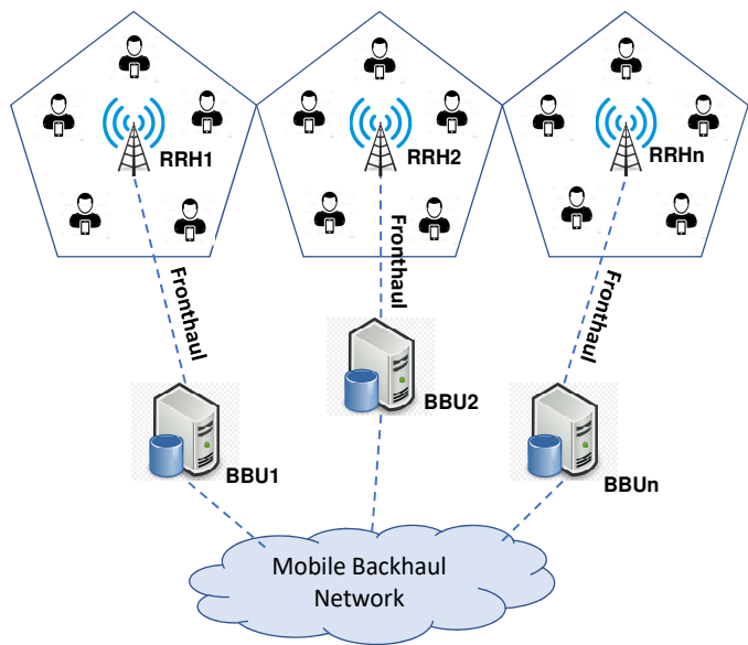
Fig. 2. D-RAN Architecture.
