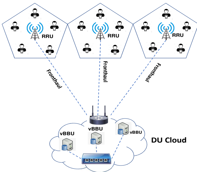
Fig. 4. vRAN Architecture.
