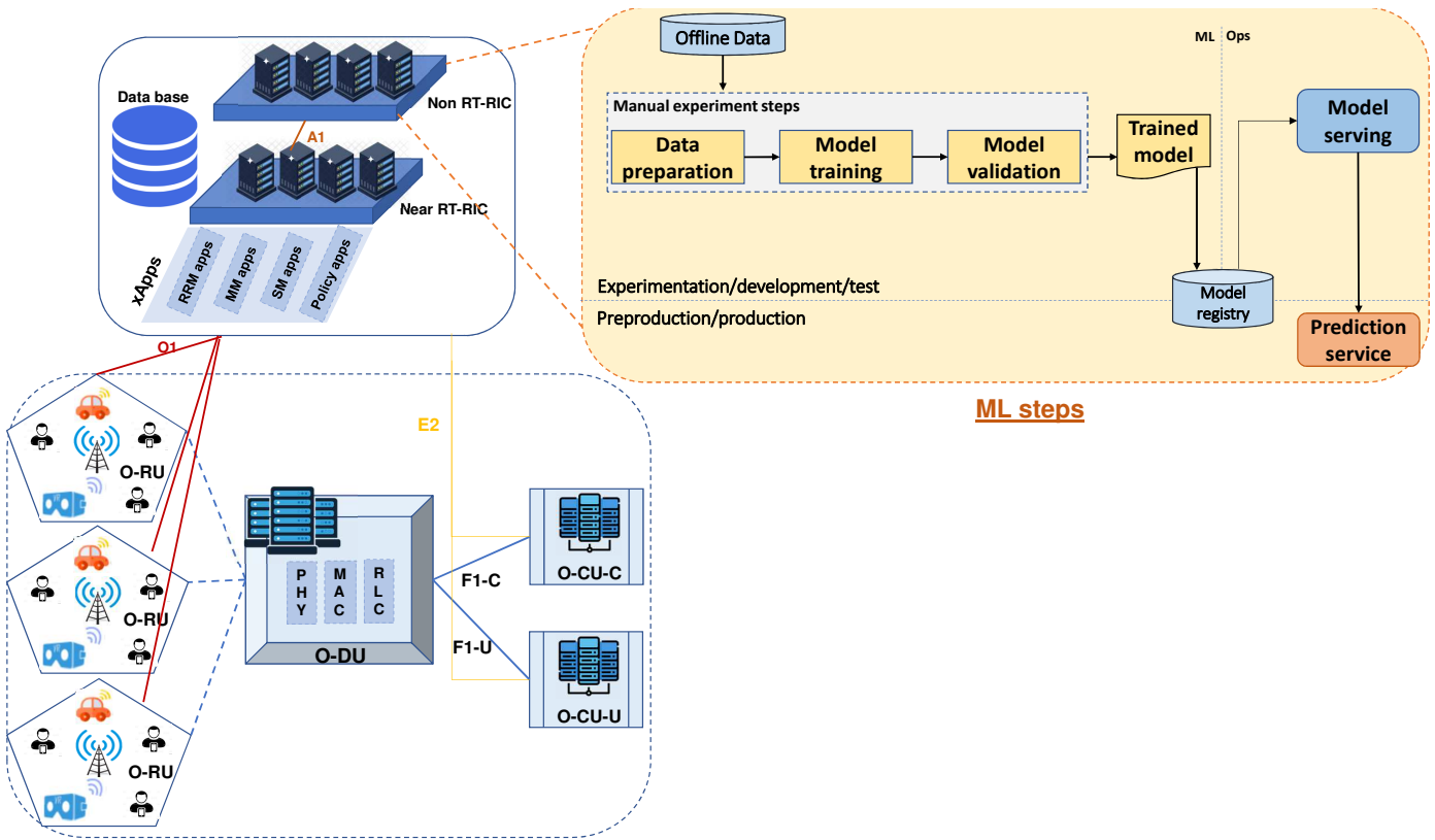
Fig. 10. Manual ML Process in O-RAN.
