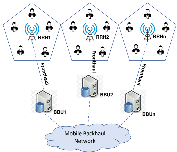
Fig. 2. D-RAN Architecture.
