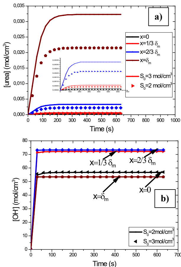
Figure 10. a) Urea concentration profiles b) OH - concentration profiles: in the enzyme membrane with S_0=2 \text{ mol/cm}^3 and S_0=3 \text{ mol/cm}^3 for V_{\max}=2.46 \text{ } \mu\text{S/cm.s} , K_m=19.01 \cdot 10^{-7} \text{ mol/cm}^3 , \delta_d=0.002 \text{ cm} , \delta_m=0.02 \text{ cm} , D_{sd}=2 \cdot 10^{-8} \text{ cm}^2/\text{s} , D_{sm}=4 \cdot 10^{-7} \text{ cm}^2/\text{s} , D_{pd}=10^{-22} \text{ cm}^2/\text{s} and D_{pm}=7 \cdot 10^{-8} \text{ cm}^2/\text{s} .
