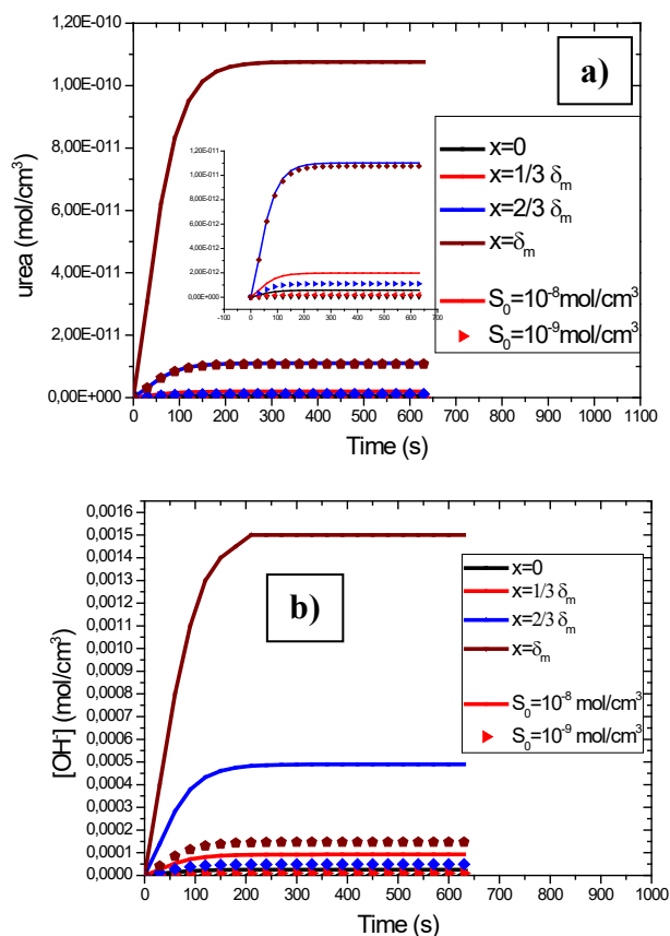
Figure 11. a) Urea concentration profiles b) OH - concentration profiles: in the enzyme membrane with S_0=10^{-8} \text{ mol/cm}^3 and S_0=10^{-9} \text{ mol/cm}^3 for V_{\max}=2.46 \text{ } \mu\text{S/cm.s} , K_m=19.01 \cdot 10^{-7} \text{ mol/cm}^3 , \delta_d=0.002 \text{ cm} , \delta_m=0.02 \text{ cm} , D_{sd}=2 \cdot 10^{-8} \text{ cm}^2/\text{s} , D_{sm}=4 \cdot 10^{-7} \text{ cm}^2/\text{s} , D_{pd}=10^{-22} \text{ cm}^2/\text{s} and D_{pm}=7 \cdot 10^{-8} \text{ cm}^2/\text{s} .
