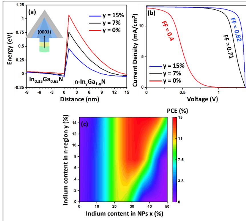
Figure 4. (a) Conduction band at the hetero-junction along the line in [0001] direction as shown in schematic, (b) J–V characteristics under AM1.5 illumination for the p-GaN/ \text{In}_{0.35}\text{Ga}_{0.65}\text{N} /n- \text{In}_y\text{Ga}_{1-y}\text{N} NP-C structure and (c) PCE with respect to Indium content in NPs (x) and n-region (y).
