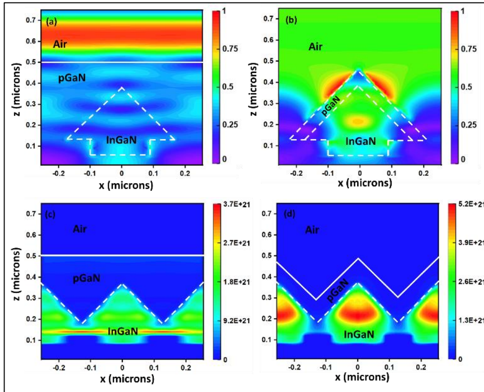
Figure 3. Cross-section ( x, z ) maps of the normalized optical electric field intensity obtained at x = 30\% and \lambda = 525 nm for (a) NP-L and (b) NP-C structures. Optical absorption has not been taken into account to clearly highlight the light trapping effect. Photogeneration rate maps ( \text{cm}^{-3} \cdot \text{s}^{-1} ) averaged along the y -axis for (c) NP-L and (d) NP-C at x = 30\% .
