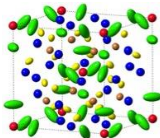
Figure 1. Perspective view of the crystal structure of Cu 12 Sb 4 S 13 in the ellipsoidal representation (drawn at the 95% probability level). The Cu1 and Cu2 atoms are in blue and green, respectively. Sb atoms are shown in brown while S1 and S2 atoms are in yellow and red, respectively.
