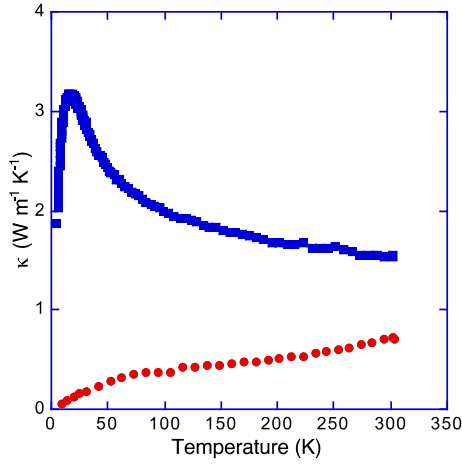
Figure 7. Temperature dependence of the total thermal conductivity of the tetrahedrites Cu 12 Sb 2 Te 2 S 13 (red filled circles) and Cu 10 Te 4 S 13 (blue filled squares). Adapted from Ref. 46 with permission from the PCCP Owner Societies.
