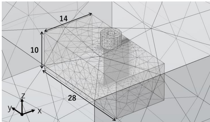
Fig. 4 Numerical model.
