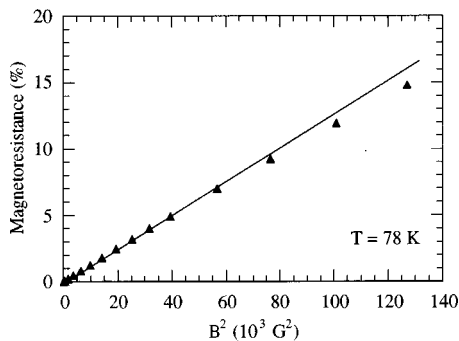
FIG. 2. Magnetoresistance in the binary direction of sample No. 2 (Table II) as a function of magnetic field B parallel to the trigonal axis for T = 78 K. The low-field condition (solid line) is observed up to a value of 200 G. The slope at low fields gives A_{13} .
