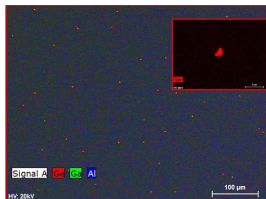
Fig.1 EDX map of a sample of nominal composition Al 0.36 Ga 0.64 N. Ge crystallites appear in red (zoom given in inset)
