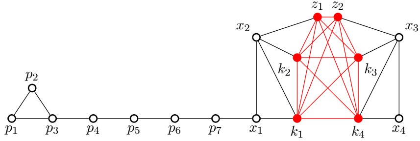
Figure 2: An interval graph G containing the complete graph K_6 (represented by the red vertices and edges). Observe that the maximum clique of G does not contain a single simplicial vertex.
