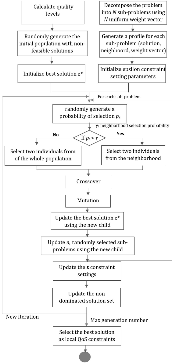
FIGURE 7. MOEA overview
