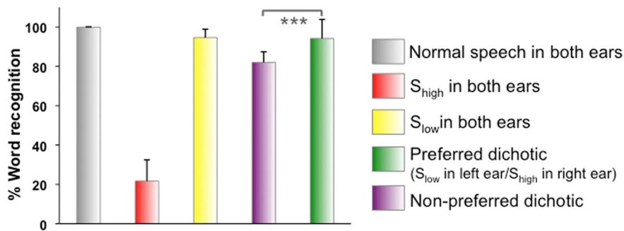
Figure 2. Behavioral results of Experiment 1. Percentage of speech recognition (whole-word scoring). *** indicate t -test with p < 0.001 .
