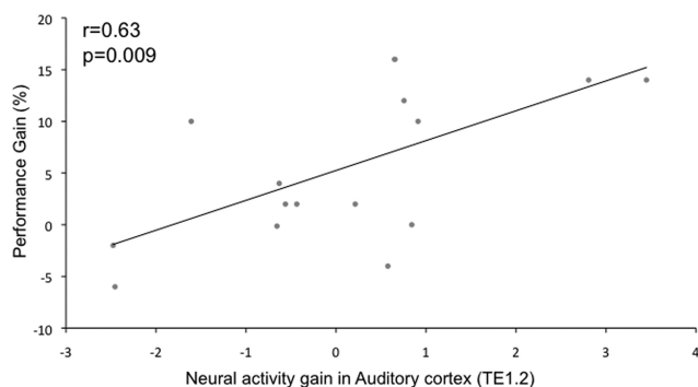
Figure 6. Positive correlation between neural activity gain measured from cytoarchitectonic region TE1.2 (fMRI experiment, S_{high} in left ear/ S_{low} in right ear minus S_{low} in left ear/ S_{high} in right ear) and performance gain (difference in speech recognition score between the two dichotic conditions).
