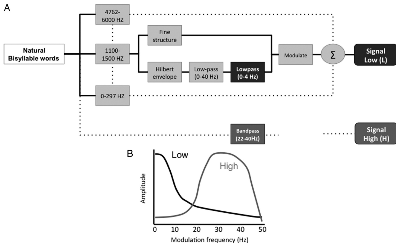
Figure 1. Stimuli. A , Signal processing block diagram. Signals were low-pass filtered at 6 kHz, sampled at 16 kHz, and quantized with 16-bit resolution. The frequency spectrum of the speech signal was partitioned into 14 frequency bands with a linear-phase finite impulse response filter bank (slopes 60 dB/100 Hz or greater), spanning the range 0.1–6 kHz, spaced in 1/3 octave steps (approximately critical band-wide) across the acoustic spectrum. The Hilbert transform was used to decompose the signal in each band into a slowly varying temporal envelope and a rapidly varying fine structure. The temporal envelope was subsequently low-pass filtered with a cutoff frequency of 40 Hz and then either low- (0–4 Hz) or band- (22–40 Hz) pass filtered. The time delays, relative to the original signal, introduced by the filtering, were compensated by shifting the filter outputs. After the filtering, the envelope was combined with the carrier signal (fine structure) by multiplying the original band by the ratio between the filtered and original envelopes. The result for each original signal ( S ) is S_{\text{low}} and S_{\text{high}} , containing only low- or high-modulation frequencies. B , Schematic representation of modulation spectrum for each stimulus category.
