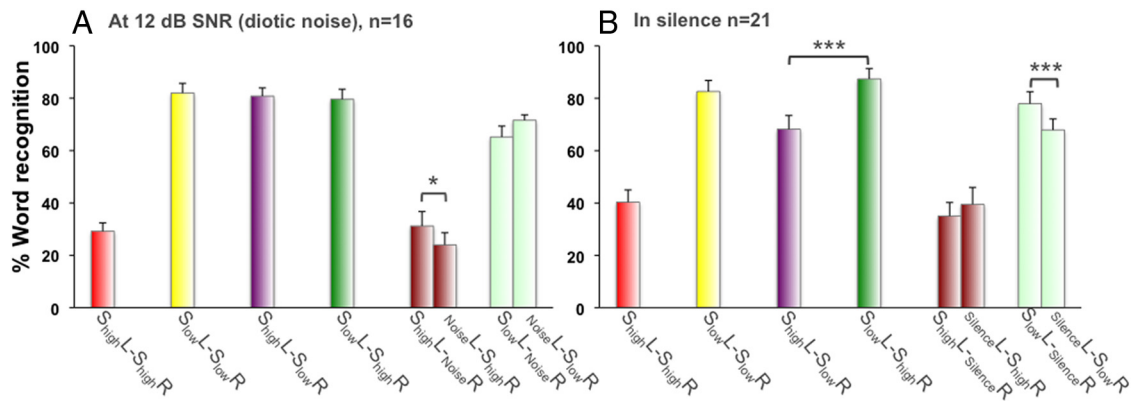
Figure 3. Behavioral results of Experiments 2 and 3. A , Experiment 2 in noise (12 dB SNR): percentage of word recognition (syllable scoring). The expected dichotic effect is absent (no difference between purple and dark). B , Experiment 3 in silence: percentage of word recognition (syllable scoring). The expected effect is present. * and *** indicate t tests with p < 0.05 and p < 0.001 , respectively.
