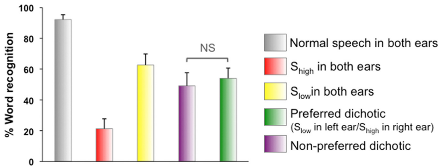
Figure 4. Behavioral results for the fMRI in Experiment 4. Percentage of speech recognition (syllable scoring). The expected dichotic effect is qualitatively present (nonsignificant).
