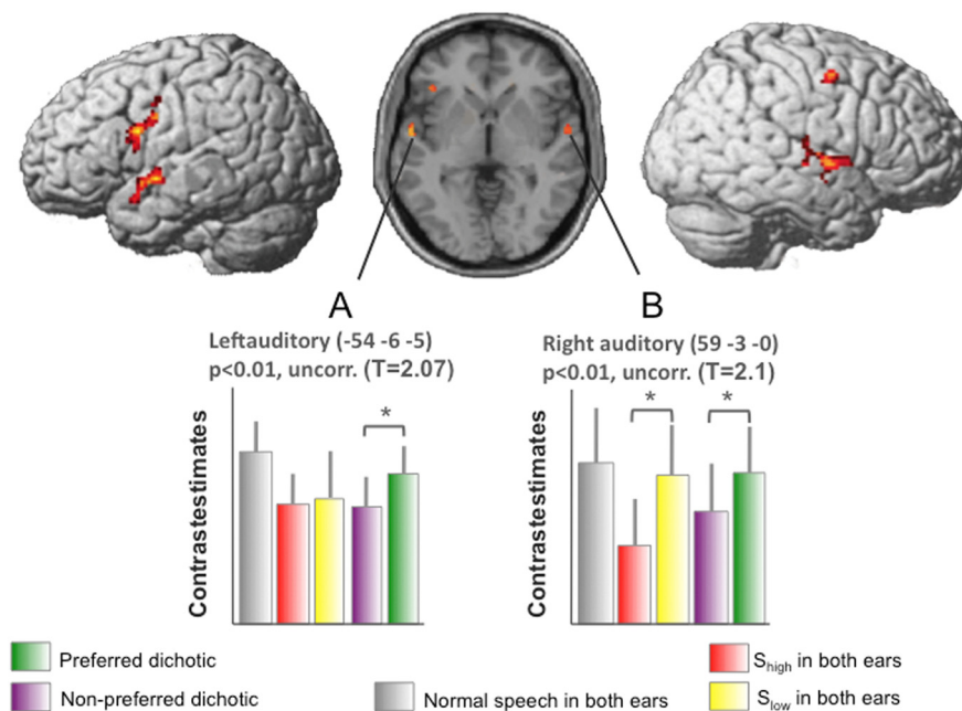
Figure 5. Whole-brain fMRI results. The preferred dichotic condition yielded more neural activity in bilateral auditory and premotor cortices. The effects remained significant after correction for multiple comparisons within the cytoarchitectonic map of auditory cortices (our hypothesis; * indicate p < 0.01 after correction), but no longer across the whole brain. Bottom, Relative level of activity across conditions in left auditory cortex ( A ) and right auditory cortex ( B ) in 1 cm spheres centered around the coordinates in parentheses.
