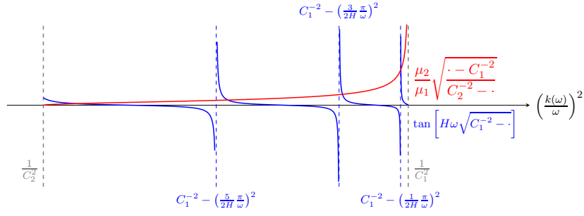
FIGURE 2. Functions \psi_1 (red) and \psi_2 (blue) when C_2^{-2} < C_1^{-2} - \left(\frac{3}{2H} \frac{\pi}{\omega}\right)^2 .
