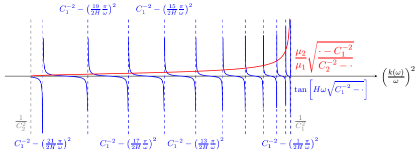
FIGURE 3. Functions \psi_1 (red) and \psi_2 (blue) when C_2^{-2} < C_1^{-2} - \left(\frac{3}{2H} \frac{\pi}{\omega}\right)^2 , but for an \omega larger than in Figure 2.
