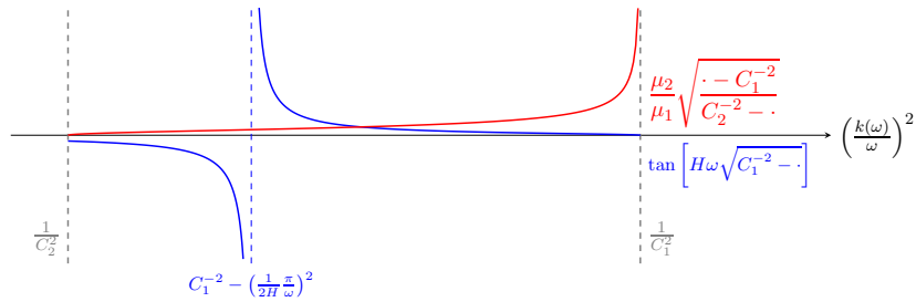
FIGURE 4. Functions \psi_1 (red) and \psi_2 (blue) when C_1^{-2} - \left(\frac{3}{2H} \frac{\pi}{\omega}\right)^2 < C_2^{-2} < C_1^{-2} - \left(\frac{1}{2H} \frac{\pi}{\omega}\right)^2 .
