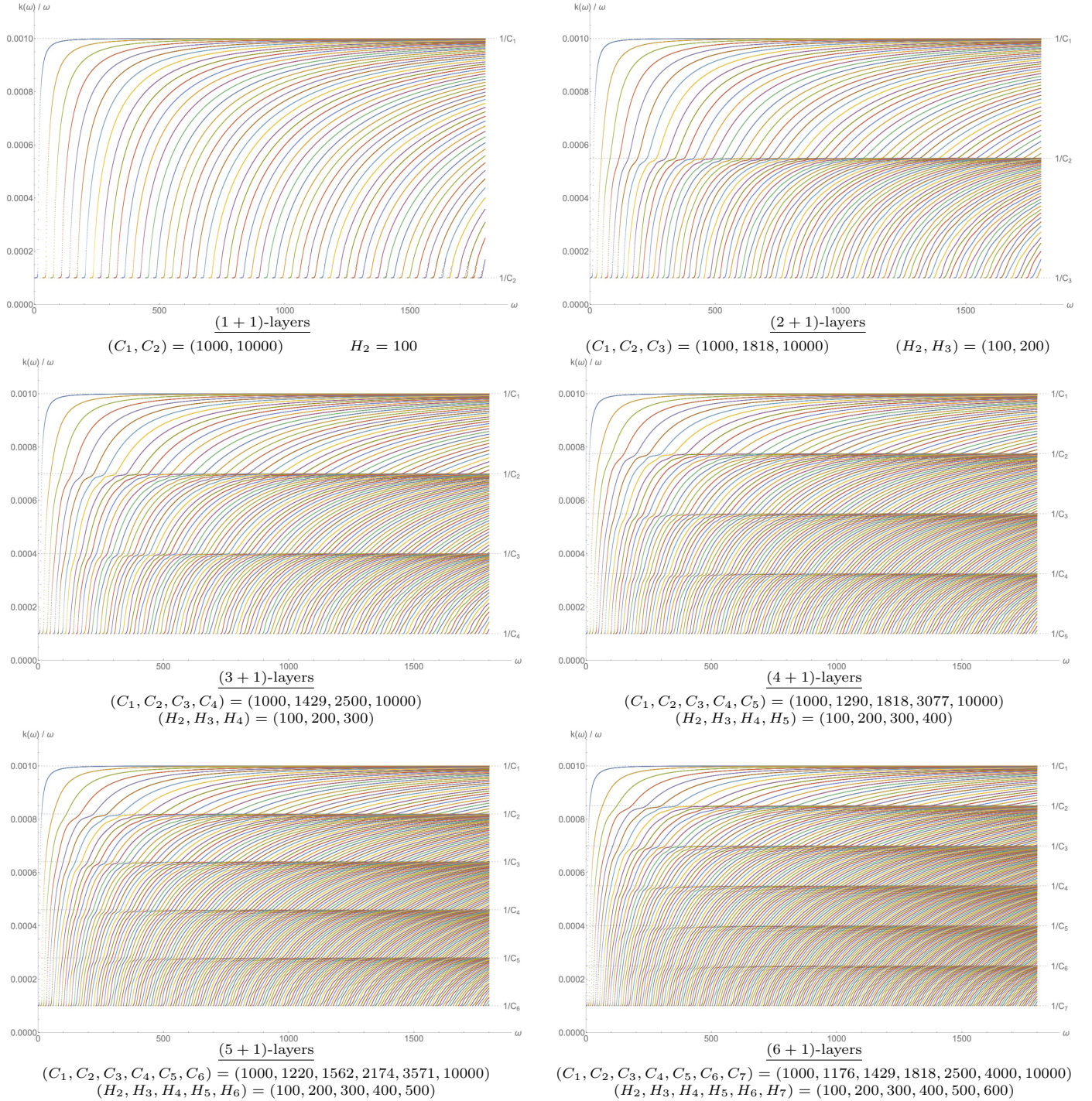
FIGURE A. Numerical computations of \omega \mapsto \{k_\ell(\omega)/\omega\}_\ell , from 1 + 1 to 6 + 1 layers.
