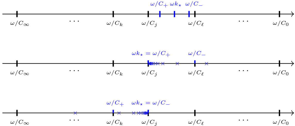
FIGURE 1. Sketch of the definition of C_\pm . Top: k_* \neq 1/C_j for all j . Center & bottom: k_* = 1/C_j for some j , the two subcases.
