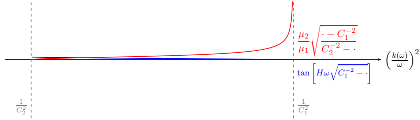
FIGURE 5. Functions \psi_1 (red) and \psi_2 (blue) when C_1^{-2} - \left(\frac{1}{2H} \frac{\pi}{\omega}\right)^2 < C_2^{-2} ( \omega small).
