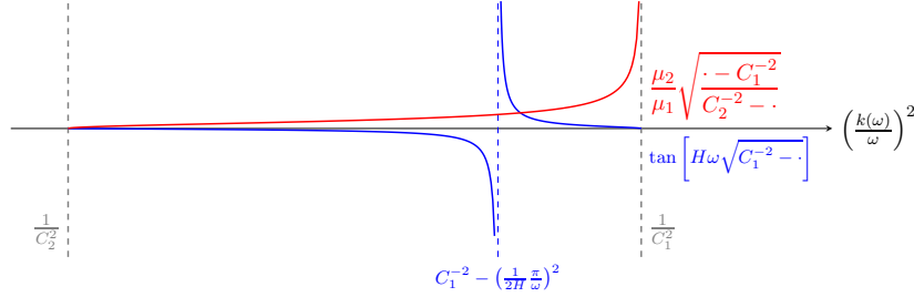
FIGURE 6. \omega = \omega_2 .
