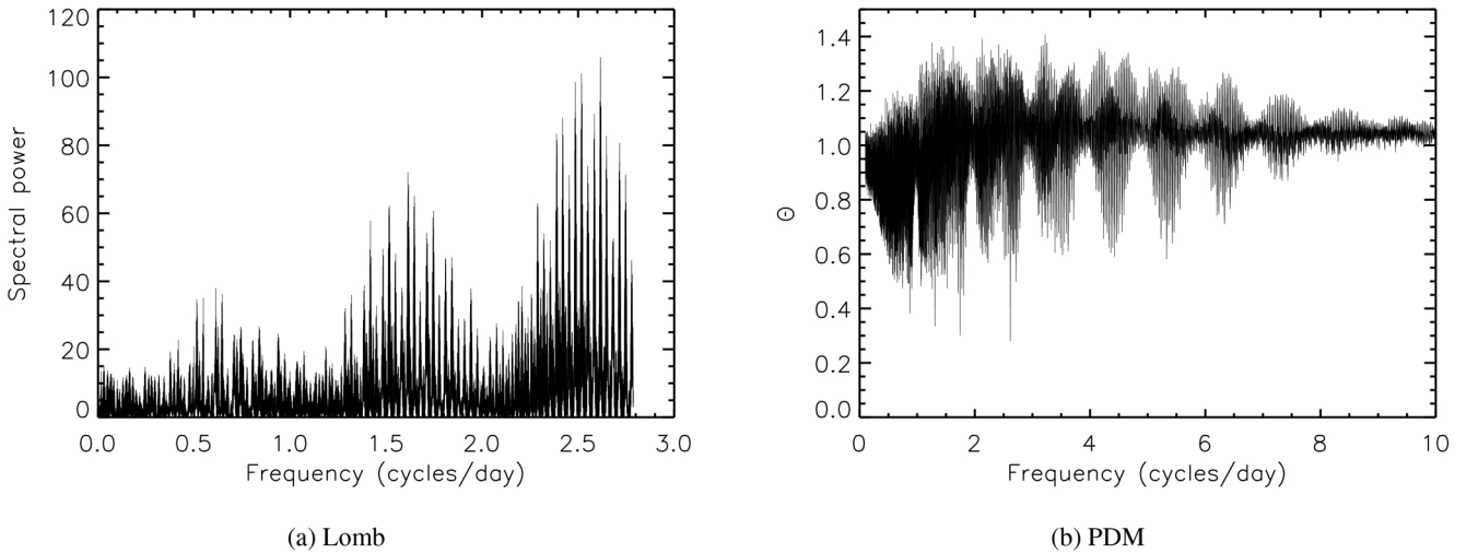
Fig. 3. (a) Lomb periodogram spectral power derived from 2014, 2015, and 2019 photometric data. The spectral power is plotted as a function of the frequency (cycles per day). The maximum spectral power of 106 is at 2.61670 cycles per day, which corresponds to a rotation period of 9.1718 h. (b) PDM plot derived from 2014, 2015, and 2019 photometric data. The minimum value of \theta is given for a frequency of 2.61669 cycles per day (i.e., P = 9.17188 h).
