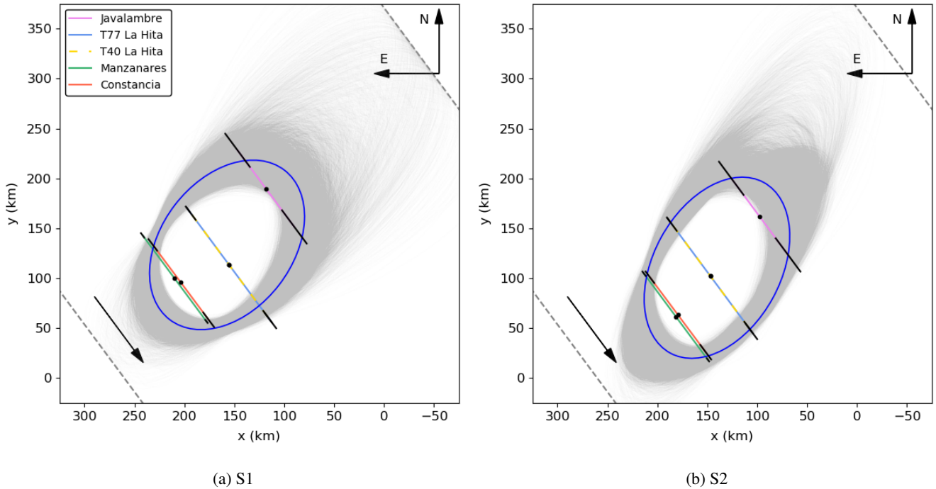
Fig. 5: Elliptical fit to the five occultation chords obtained from the light curves shown in Figure 2, where x and y depict the distances in the sky plane in the East-West and North-South directions respectively. The gray shadowed region represents the 10,000 ellipses given by the Monte Carlo method, with the blue ellipses representing the best fit to the extremities of the chords by least-squares minimization of the geometric distances. For reference, the colours of the chords match those of Figure 2, with the black solid lines in the extremities representing the 1\text{-}\sigma uncertainties of the ingress/egress times. We note that La Hita T40's and T77's chords are overlapping one another. gray dashed lines outside the ellipse represent the closest locations (to the North and South of the object) where the stellar occultation was not detected, which correspond to the data from Agrupación Astronómica de Sabadell (Sabadell) and La Sagra (Granada). Black arrows at the left-bottom corner indicate the star's motion relative to the centaur. (a) Manzanares's chord is displaced to match Constancia's ingress (S1 fit). (b) All chords' centers are aligned (S2 fit).
