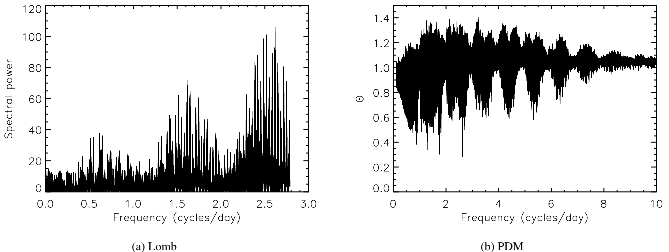
Fig. 3: (a) Lomb periodogram spectral power derived from 2014, 2015, and 2019 photometric data. The spectral power is plotted as a function of the frequency (cycles/day). The maximum spectral power of 106 is at 2.61670 cycles/day, which corresponds to a rotation period of 9.1718 h. (b) PDM plot derived from 2014, 2015, and 2019 photometric data. The minimum value of \theta is given for a frequency of 2.61669 cycles/day (i.e., P = 9.17188 h).
