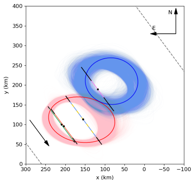
Fig. 6: Simultaneous fit of two ellipses to the five chords from the light curves in Figure 2 where x and y depict the difference between the JPL orbit and the center of the shadow. (No shift to the chords has been applied other than Manzanares' due to the error in the computer synchronization). The blue and red ellipses represent the best fit in terms of minimization of a \chi^2 function, with the blue and red shadowed regions representing all 10,000 possible solutions given by the Monte Carlo method. For reference, the colours of the chords match those of Figure 2, with the black solid lines in the extremities representing the 1-\sigma uncertainties of the ingress/egress times. We note that La Hita T40's and T77's chords are overlapping one another. gray dashed lines outside the ellipses represent the closest locations (to the North and South of the object) where the stellar occultation was not detected, which correspond to the data from Agrupación Astron'omica de Sabadell (Sabadell) and La Sagra (Granada). The black arrow at the left-bottom corner depicts the shadow motion.
