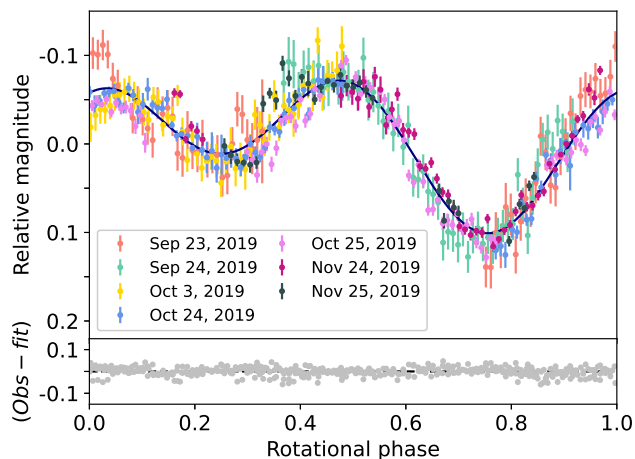
Fig. 4: Bienor’s rotational light curve was obtained using data from the 1.23-m and 1.5-m telescopes (see Section 5 for a detailed explanation on the telescopes used here). The data were folded using a rotational period of 9.1719 \pm 0.0002 h, being the zero rotational phase at the time of the occultation. Different colours represent different observation nights as described by the legend. The blue line represents a second-order Fourier-function fit to the observational data, the peak-to-valley amplitude of the fit has a value of 0.172 \pm 0.003 mag. At the bottom panel, gray dots represent the residual of the fit to the observational data, with a standard deviation of 0.02 mag.
