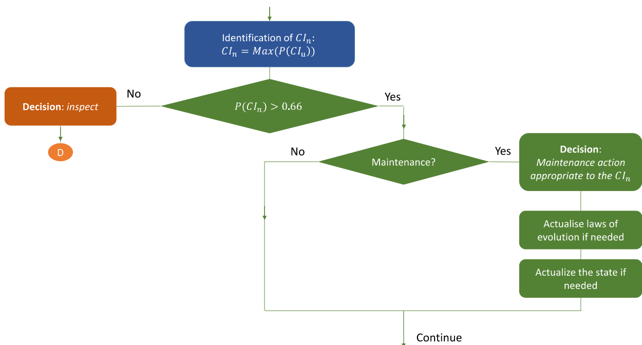
Figure A3. Flowchart of the decision process.
