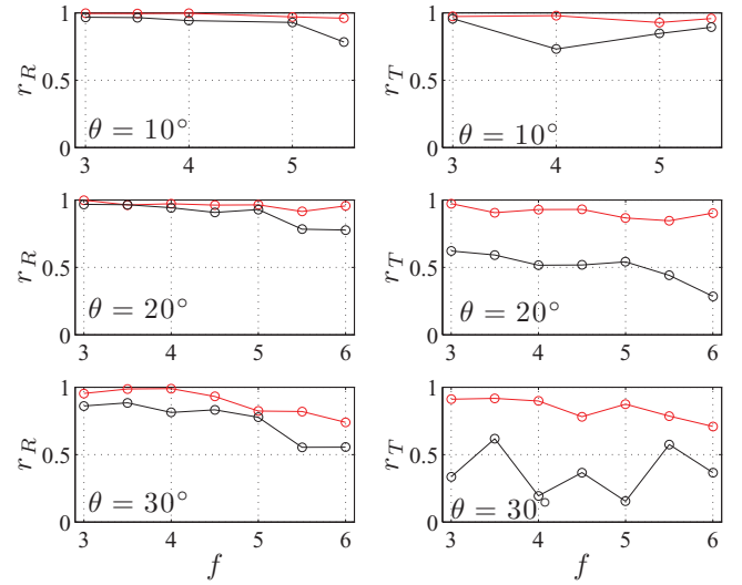
FIG. 5. (Color online) Contribution of mode 0 to the total field: left column, r_R in reflection ( X < 0 ) and right column, r_T in transmission ( X > 0 ) as a function of frequency. Red curves for the metamaterial waveguide and black curves for the reference empty waveguide.
