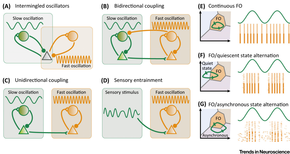
Figure 1. Architectures for Cross-Frequency Neural Coupling. (A–D) Cross-frequency coupling (CFC) architectures. (A) Intertwined oscillators. Neural oscillations in distinct frequency bands are generated by partially overlapping neural populations. In the depicted example, excitatory neurons (represented by the triangle) participate in the generation of both a slow oscillation (SO) and a fast oscillation (FO), whereas separate inhibitory populations (represented by green and orange circles) are involved in the generation of respectively SO and FO. CFC arises through the dynamics of the neural population common to both oscillations. Intermingled CFC has been proposed to explain the emergence of theta/gamma coupled oscillations in hippocampus [6,30,100], where a common excitatory population is coupled to fast-spiking (FS) cells (generating gamma oscillations) and oriens-lacunosum moleculare (O-LM) cells (generating theta oscillations). (B) Bidirectional coupling. Segregated populations are implicated in the generation of the SO and FO (in the depicted example, a population of excitatory and inhibitory neurons for both oscillations), and coupling is mediated by reciprocal coupling between SO neurons and FO neurons. This architecture was used in the first computational model of coupled theta–gamma oscillations in hippocampus, which featured two coupled inhibitory subpopulations with distinct GABA decay time [101]. Moreover, precise spiking and local field potential (LFP) dynamics of in vitro cortical slices was explained by a sophisticated model whereby a beta1 rhythm concatenates two bidirectionally coupled oscillations, a gamma rhythm generated in superficial layers and a beta2 rhythm generated in deep layers [102,103]. (C) Unidirectional coupling. Distinct populations are implicated in the generation of SO and FO, and coupling arises through one population projecting onto the other population (here SO to FO). In a recent model of speech perception in auditory cortex, coupled theta–gamma oscillations were modeled by two separate excitatory–inhibitory subpopulations responsible for the generation of both rhythms [39], with the theta module projecting onto the gamma module. (D) Sensory entrainment. Sensory entrainment of neural oscillators is a special case of unidirectional coupling where a neural oscillator is modulated by slow modulations in sensory stimulus (e.g., visual rhythmic movements or amplitude-modulated sounds). This model has been tested in the context of visual processing: a PING module generating broad gamma rhythm responds to visual activity experimentally recorded in monkey thalamus that carries strong slow modulations [28]. (E–G) Temporal dynamics of FO. (E) Continuous FO. (Left) Schematic phase diagram of FO dynamical state: continuous FO occurs when SO modulation shapes a trajectory within the region of existence of FO. (Right) The continuous model of CFC from Fontolan et al. [16] (see their Figure 5) was transformed into a mathematically equivalent model of quadratic-and-fire neurons and simulated (with membrane white noise of variance 0.01). SO is modeled as a simple modulatory signal while FO is composed of a population of pyramidal and inhibitory cells generating gamma oscillations through the PING mechanism. (Top right) SO modulating signal. (Bottom right) raster plot of FO spikes: pyramidal neurons ( n = 50 , light orange); inhibitory neurons ( n = 50 , dark orange). FO spiking occurs throughout the SO cycle. (F) Oscillation/quiescent-state intermittent FO. (Left) This type of intermittent FO occurs when SO modulation shapes a trajectory between the oscillatory and quiescent regions of FO. (Right) The intermittent model of CFC from [16] (see their Figure 7) was transformed into network of quadratic-and-fire neurons and simulated. FO alternates between a period of gamma oscillations when excitation from SO is large enough, and a quiescent state when SO signal is lower. (G) Oscillation/asynchronous-state intermittent FO. (Left) This type of intermittent FO occurs when SO modulation shapes a trajectory between the oscillatory and asynchronous regimes of FO. (Right) We modified the parameters of the gamma network of [16] (constant current, synaptic conductance, and membrane noise) such that the network alternates within SO cycle between a period of strong oscillation and a period of asynchronous spiking activity.
