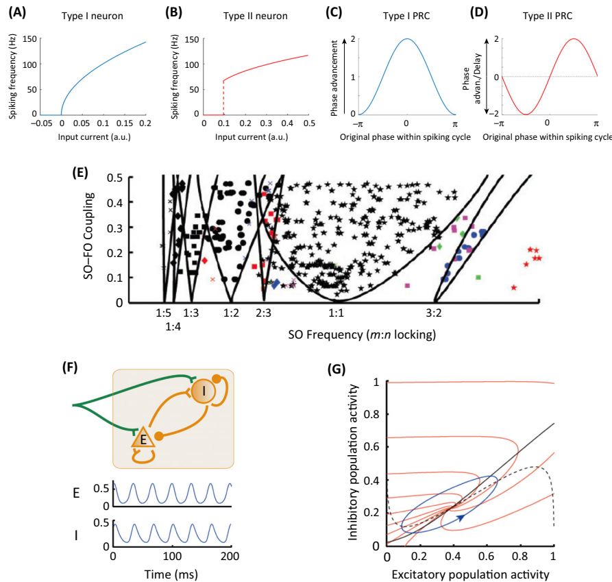
Figure 1. (A,B) Spiking frequency of type I and type II neurons as a function of driving-current magnitude. (A) Cells with type I membrane excitability can spike at any arbitrary frequency once passed beyond the bifurcation point. (B) When a type II neuron goes through the bifurcation point it starts firing from a finite frequency. (C) Phase response curve of a type I neuronal oscillator: any small excitatory input induces a phase advance within the spiking cycle of the oscillator. (D) Phase response curve of a type II neuron: an excitatory pulse either advances or delays the next spike depending on the particular phase at which the input arrives within the spiking cycle. (E) When solicited with an external sinusoidal input (SO), individual neurons from Aplysia display Arnold tongue maps (i.e., different forms of m:n coupling depending on the input frequency and amplitude). Experimental results are in fair agreement with model simulations (adapted from [29]). (F,G) Phase-amplitude coupling modeled through a set of Wilson–Cowan equations to represent the activity of a specific population of interneurons in rat hippocampus (adapted from [96]). Experimenters recorded the response of excitatory and inhibitory neurons to sinusoidal inputs induced using optogenetics tools. (F) Schematic illustration of the excitatory–inhibitory hippocampal network and spontaneous FO visible in E and I population activity in absence of external noise. (G) Phase portrait of the FO model showing the stable limit cycle of the system (blue), the nullclines (i.e., the points where either the excitatory or the inhibitory activity would be constant; black: dashed, excitatory; solid, inhibitory), and the isochrones (the set of initial points from which the dynamics would evolve towards oscillations having the same phase; red). Phase and amplitude modulations of FO can be inferred from the phase portrait, given a specific set of initial conditions.
