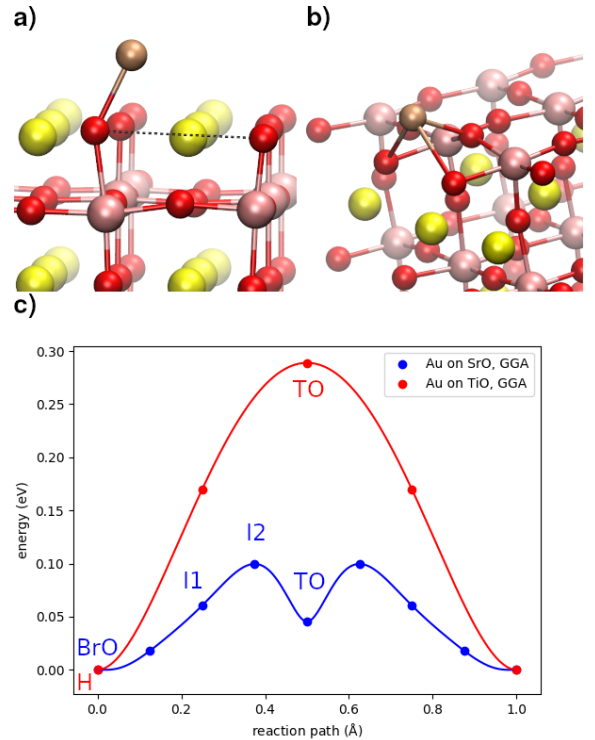
Figure 2: a) TO minimal configuration of an Au adatom on SrO-terminated STO. b) H minimal configuration of Au on TiO 2 -terminated STO. c) Lowest energy paths of Au adatoms on a SrO (blue) and a TiO 2 (red) -terminated STO surface.
