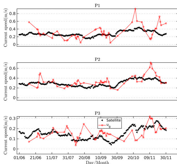
FIG. 5. Comparison of time series for u_g (N4) vs satellite-derived geostrophic current speed for the three stations along the latitudinal axis of the HFR domain. Red color for HFR and black color for satellite.
