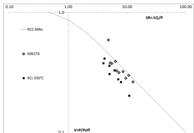
Fig. 6. RCC-MRx efficiency diagram for austenitic stainless steels compared to experimental effective primary stresses of tests performed on 6061-T6 aluminium alloy and Mod 9Cr-1Mo steel, from [9].
