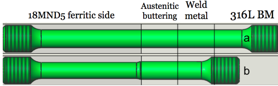
Figure 4: Machining of tensile specimens in a SS DMW mock-up : (a) crossweld specimen with homogeneous diameter and (b) crossweld specimen with variable diameter
