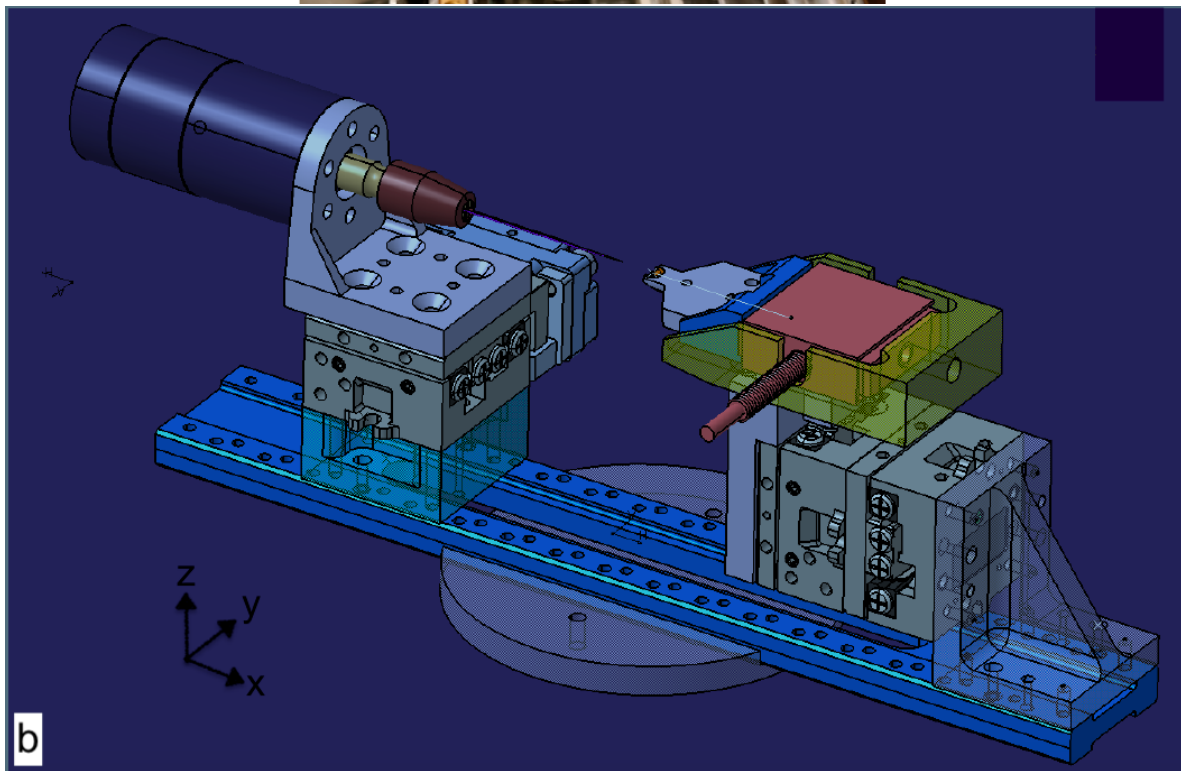
Figure 8: (a) In-situ micro-tensile testing machine (b) 3D representation of the in-situ micro-tensile testing machine.
