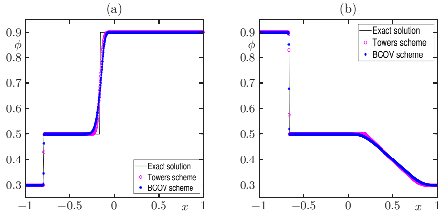
FIGURE 3. Example 1: numerical solution of solution with M = 800 and comparison with the exact solution of the Riemann problem (a) with \phi_L = 0.3 and \phi_R = 0.9 at simulated time T = 1.8 , (b) with \phi_L = 0.9 and \phi_R = 0.3 at simulated time T = 1.5 . Here and in Figures 4 and 5 we label with ‘Towers scheme’ the scheme (1.7) proposed in [28] and by ‘BCOV scheme’ the scheme of Algorithm 2.1 advanced in the present work.
