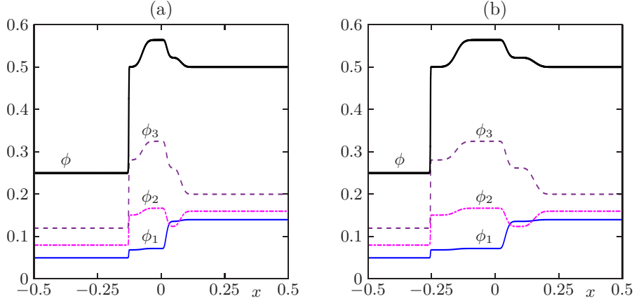
FIGURE 8. Example 5: numerical solution for a congested flow regime ( \mathcal{G}(t) = 0 ): density profiles with M = 1600 at simulated time (a) T = 0.1 , (b) T = 0.2 . The initial condition is the same as in Figure 7 (a).
