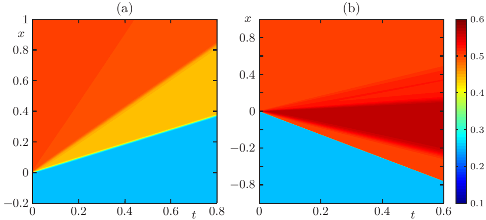
FIGURE 9. Example 5: simulated total density computed with BCOV scheme with N = 3 and M = 1600 : (a) free flow ( \mathcal{G}(t) = \alpha_V ), (b) congested flow ( \mathcal{G}(t) = 0 ).
