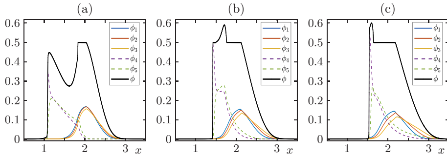
FIGURE 14. Example 7: numerical solution at three different time computed with BCOV Scheme with M = 12800 and N = 5 . (a) t = 0.1 . (b) t = 0.2 . (c) t = 0.3
