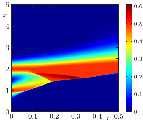
FIGURE 15. Example 7: simulated total density computed with BCOV scheme with N = 5 and M = 1600 at simulated time T = 0.5 .
