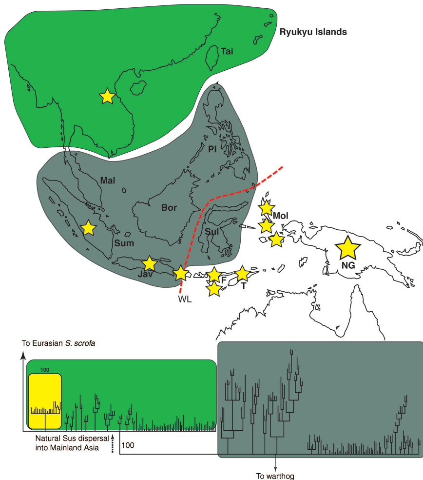
Fig. 1. Bayesian (Monte Carlo–Markov chain) consensus tree of 249 Sus mtDNA control region haplotypes rooted by a common warthog ( Phacochoerus aethiopicus ). Gray (basal) and green (derived) clusters on the tree correspond to general regions on the map where the majority of pigs possess haplotypes within that cluster. The yellow clade represents the Pacific Clade. Yellow stars represent islands on which at least one specimen possessing Pacific Clade haplotypes was identified. The yellow star in Southeast Asia represents the two mainland Asian wild boar samples in Vietnam that possessed this haplotype. Regions on the map are: Mal, peninsular Malaysia; Bor, Borneo; Sum, Sumatra; Jav, Java; Sul, Sulawesi; F, Flores; T, Timor (both in the Lesser Sundas); Mol, Moluccas Islands; PI, Philippines; Tai, Taiwan; NG, New Guinea. The dashed red line labeled WL represents the Wallace Line. The black dashed arrow leading to the more derived portion of the tree illustrates the natural movement of wild Sus out of ISEA and into mainland Asia. See SI Fig. 4 for a more detailed version of the tree.
