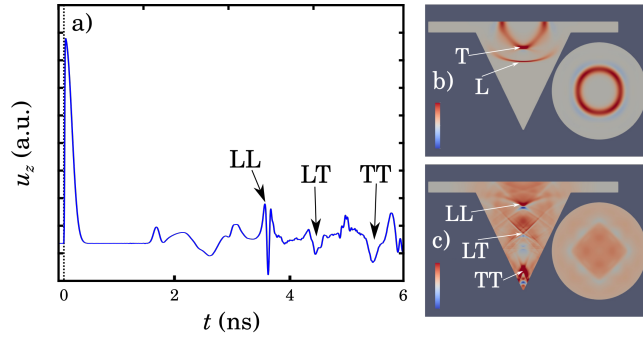
FIG. 4. (a) z -component of the displacement calculated at the back of the AFM probe at the center of the tip. Section and top view of the z -component of the displacement field in the (001) plan at (b) 0.83 ns and (c) 3.26 ns. The longitudinal and transverse waves are identified L and T respectively prior to the reflection at the tip and LL and TT after. The wave identified LT correspond to a transverse wave obtain by mode conversion from the reflection on the longitudinal wave L.
