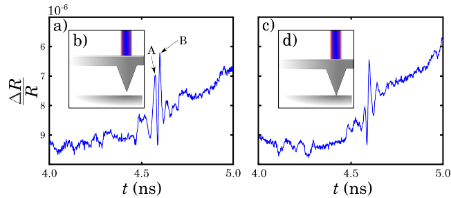
FIG. 5. Variation of reflectivity measured on the Al layer measured when (a) the AFM probe is far from the sample and (c) in contact with a silicon sample. (b) and (d) Designs of the measurement geometries.
