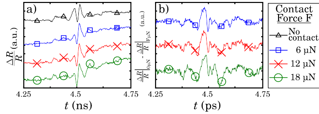
FIG. 6. (a) Comparison of the shape of the reflected echo at the end of the tip as a function of the contact force applied. (b) Subtraction with the non-contact reference. The maximum sensitivity is located on peak A and does not seem to be affected by the quality of the contact. Time t = 0 ps is an arbitrary choice and does not correspond to the arrival time of the pump pulse.
