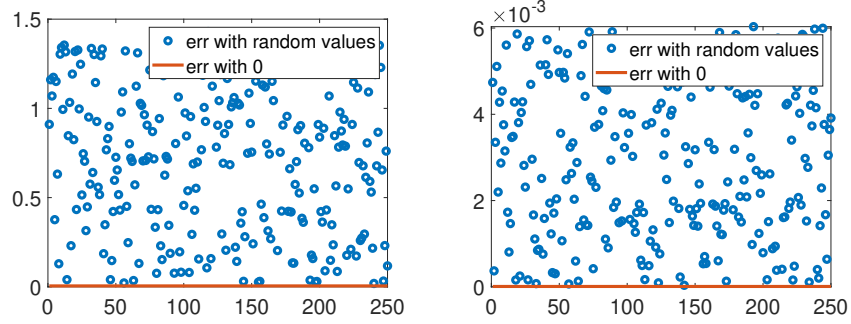
Fig. 1: Number random values between -150 and +150 generated for \sigma_{i3} VS Error (infinity norm) on \lambda at the 5th (Left) and 10th (Right) iteration using random antidiagonal elements (blue dots) or just 0 (red line).
