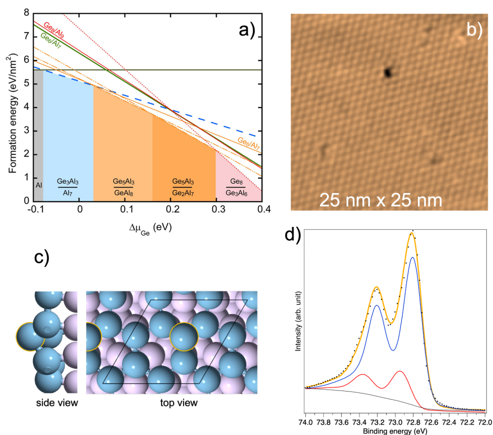
Figure 4. (a) Variation in the calculated formation energy with respect to \Delta\mu_{\text{Ge}} = \mu_{\text{Ge}} - E_{\text{Ge}} bulk for different Ge/Al(111) models. Black horizontal line: Al(111) surface. Wide lines correspond to the (\sqrt{7} \times \sqrt{7}) R \pm 19.1^\circ models (blue dashed line: \text{Ge}_3\text{Al}_3 ; green solid line: \text{Ge}_6 ), whereas narrow lines correspond to the (3 \times 3) models. (b) 25 nm \times 25 nm STM image ( U_s = -1.0 V, I = 300 pA) of a germanene overlayer grown by segregation on an epitaxial Al(111) thin film on a Ge(111) substrate; (c) Top view of the DFT-optimized models of (2 \times 2) germanene on Al(111)- (3 \times 3) with one Ge atom protrusion, namely, the hexagonal model. Ge and Al atoms are shown as blue and purple balls, respectively. The black rhombus represents the Al(111)- (3 \times 3) cell. The orange circles represent the Ge atoms shifted outward with respect to the other Ge atoms. (d) High-resolution synchrotron radiation normal emission Al 2p CL spectrum taken in highly surface-sensitive conditions at a photon energy of h\nu = 100 eV for the (2 \times 2) germanene phase on Al(111)- (3 \times 3) ; (a) Figure 4 of Zhang et al. [24], (b–d) derived from Yuhara et al. [26].
