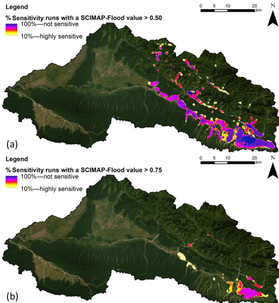
FIGURE 8 The overall sensitivity of areas having a SCIMAP-Flood value of (a) >0.50 and (b) >0.75 , based on the point density analysis of SCIMAP-Flood output across the 10 tested sensitivity scenarios (Section 2.3). Areas with no colour did not have a SCIMAP-Flood value of >0.50 . The areas in blue have a low sensitivity to the data input and feature in a greater proportion of the sensitivity runs. The yellow areas have a high sensitivity to the data input and feature in a lesser proportion of the sensitivity runs. Grid projection: WGS84 UTM Zone 45° N. Base imagery: ArcGIS Online World Imagery
