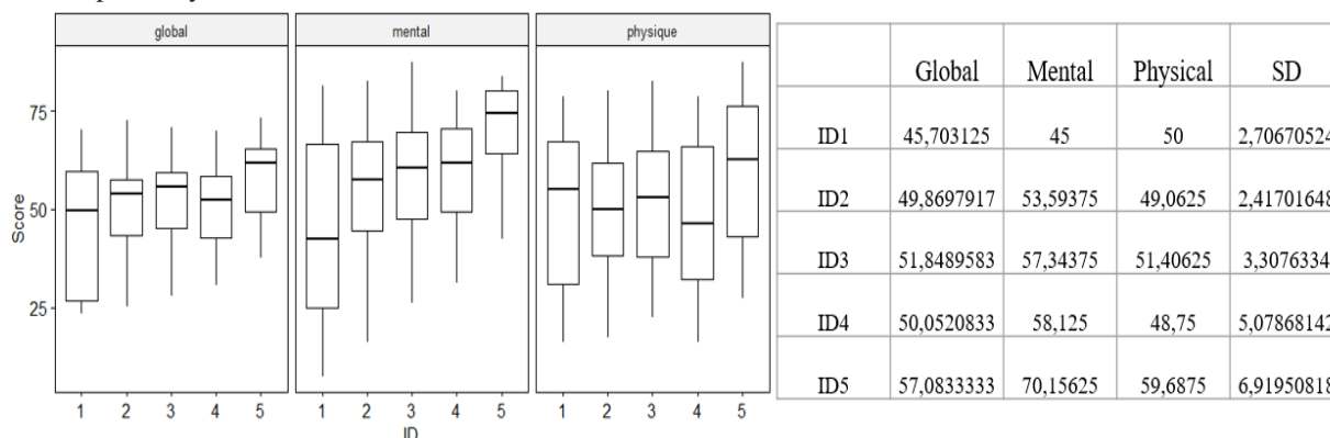
Figure 3: (A) Different NASA-TLX scores according to task difficulty. (B) Table of mean scores for all participants.
