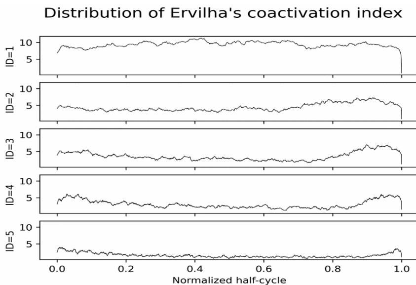
Figure 4: Distribution of the muscle co-activation index of the co-activation index for the couple biceps/triceps for all participants.
