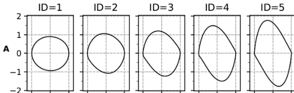
Figure 2: A-Phase plane (velocity according to position) normalized between 1 and -1 [9].
