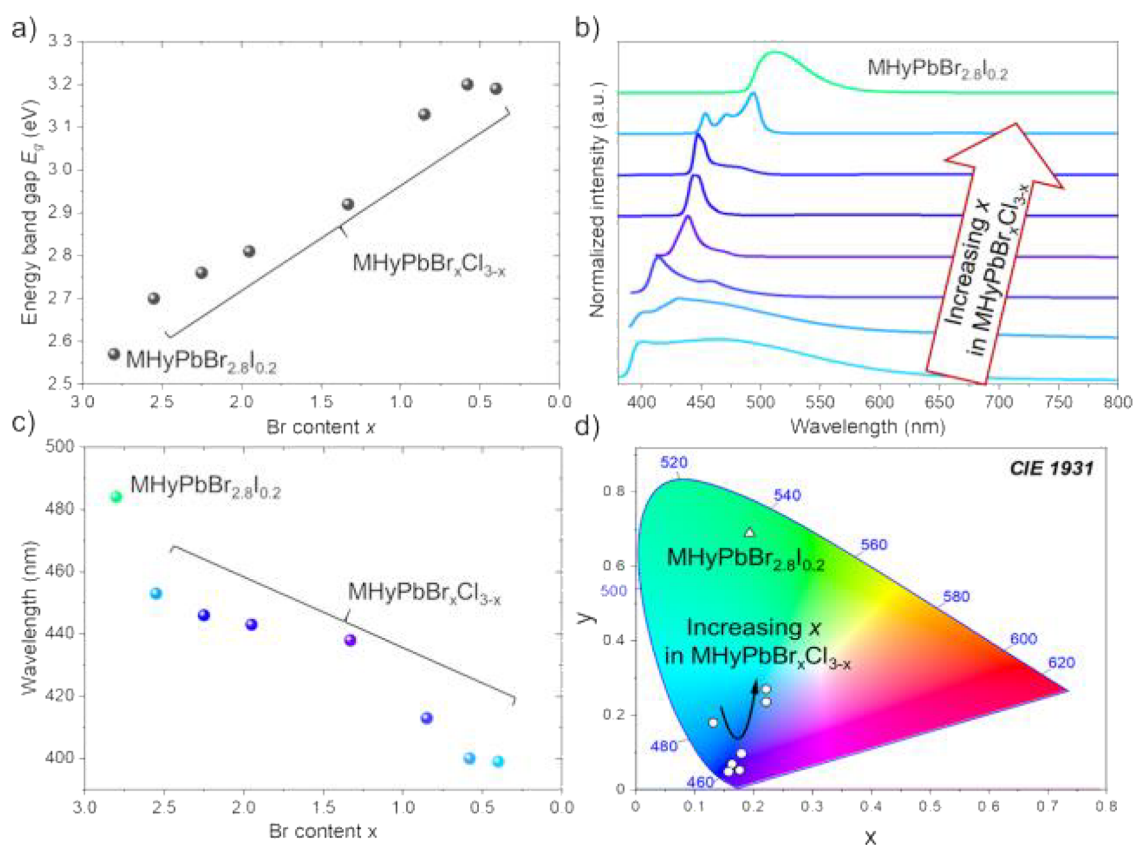
Figure 8. (a) Values of the energy band gap E_g of the investigated compounds. (b) PL spectra of MHyPbBr x Cl 3-x and MHyPbBr 2.8 I 0.2 recorded at 80 K, (c) changes of FE band position with sample composition, and (d) CIE coordinates of the investigated samples.
