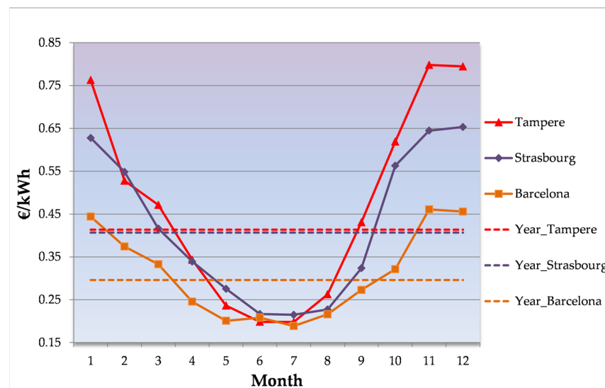
Figure 5. The exergo-economic cost of electricity on monthly and annual basis in different locations adapted from [9].
