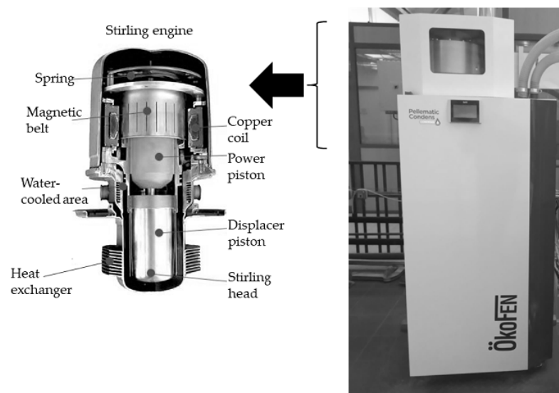
Figure 4. Stirling engine powered Pellematic Condense_e micro-cogeneration system analyzed in and adapted from [65].
