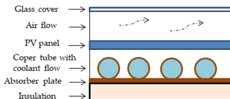
Figure 3. The cross-section of the PVT collector with water and air cooling systems adapted from [37].
