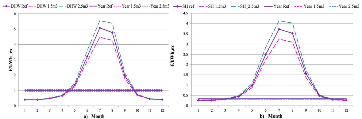
669 670 Fig. 17. The monthly and yearly exergo-economic costs of a) DHW and b) space heating with different storage capacities. 671
