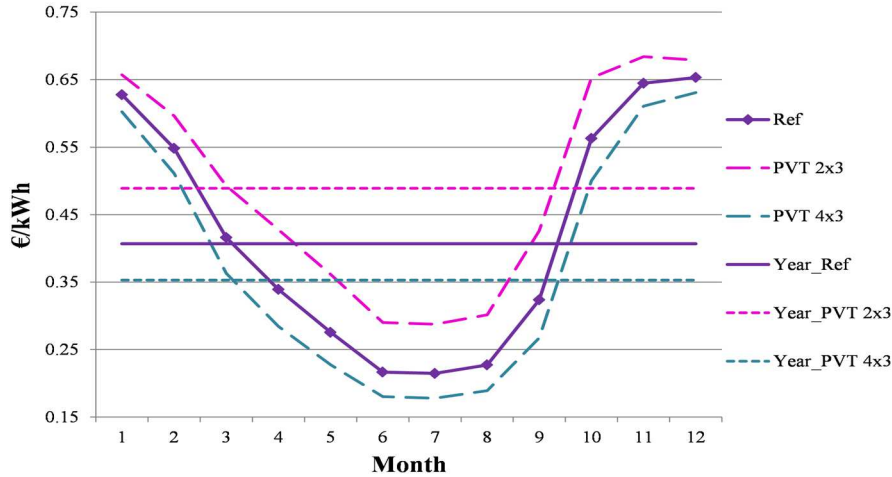
653 654 Fig. 16. The monthly and yearly exergo-economic costs of electricity produced by the hybrid energy system with different PVT capacities. 655
