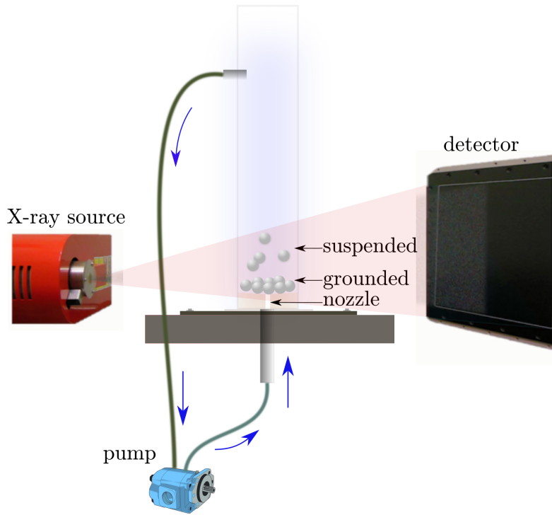
Figure 1: (color online) Schematic representation of the set-up inside the X-ray scanner. Note that the system is not rotated and radiographs are acquired only in the orientation illustrated. Spheres that are at altitudes z < d_s are labeled as grounded, while spheres at higher altitudes are deemed suspended.
