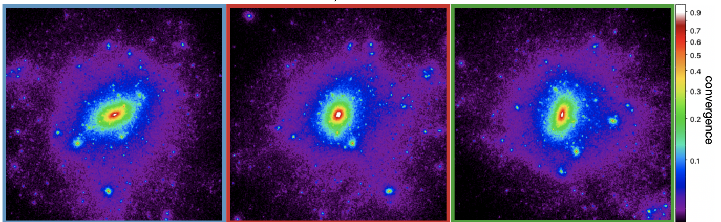
Fig. 3. Convergence maps of the three considered random projections of a cluster, namely the halo-4 at z = 0.22 . The left, central and right panels show the projections along the z , y , and x axis coordinates of the re-simulated box. The source redshift of the map is fixed at z_s = 3 . The size of the field of view is 5 Mpc ( 3.4 h^{-1} Mpc) on a side, 10 Mpc along the line-of-sight. The map resolution is 2048 pixels on a side.
