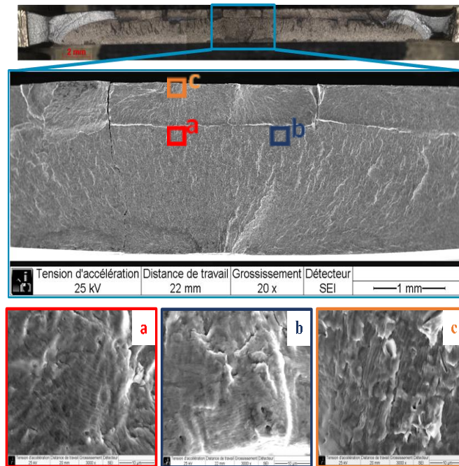
Figure 6: Macroscopic observation of fracture surface
