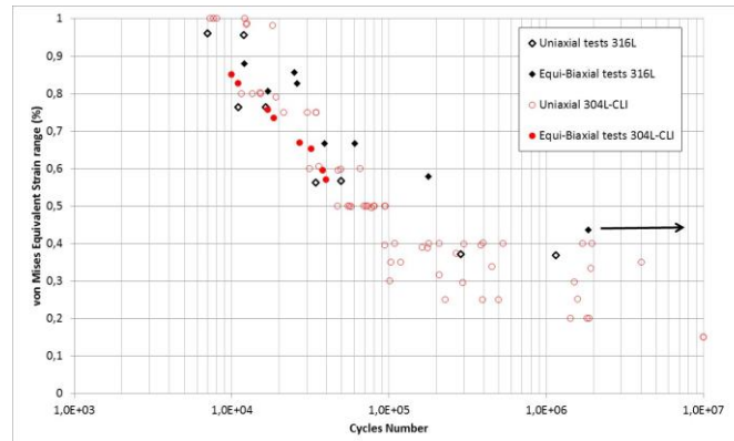
Figure 8: Fatigue data obtained on the two austenitic stainless steels (316L and 304L-CU)
