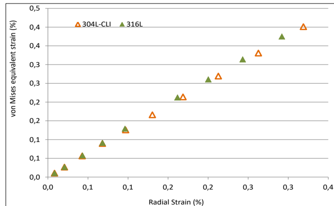
b) Determination of the equivalent strain with the "transfer" curve: radial strain versus equivalent strain
