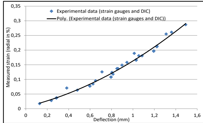
a) Calibration curve: Deflection versus radial strain
