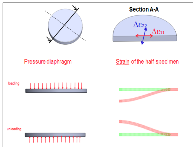
Figure 3: Principle of the first fatigue test
