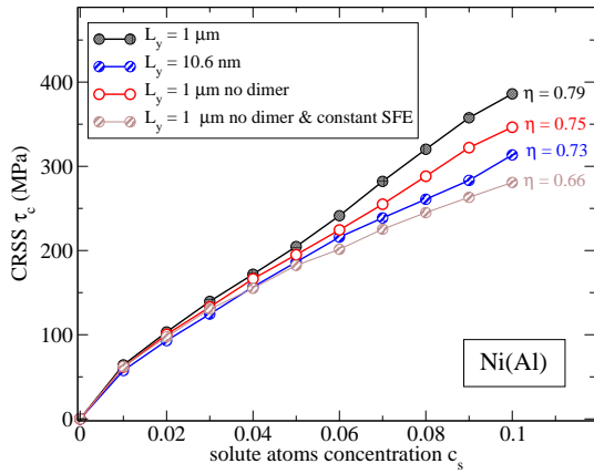
FIG. 18: ELM computations for the CRSS against solute atomic concentration c_s in Ni(Al), for different distances between the dislocation periodic images along the Y direction L_y (see legend) and for different approximations for dimers interaction potentials and the SFE. The dislocation length is L_x = 80 nm and the glide distance d_g = 100 nm. The effective concentration exponent \eta is reported for each set of data.
