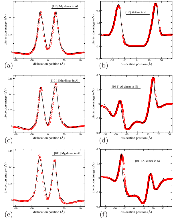
FIG. 12: Internal energy U_{\text{cell}} in ASC for an edge dislocation bypassing dimers situated in the (1\bar{1}1) planes just above the glide plane (A1) . On the left hand side Al(Mg) and on the right Ni(Al). Symbols represent the ASC data and the continuous line corresponds to ELM which the interaction potentials V_{i-n} and W_{i-n} ( i \in [II, III, IV] and n = (A1) ) have been properly adjusted on the atomistic data.
