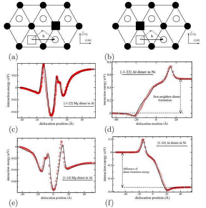
FIG. 14: In (a) and (b) schematic representation of the solute atom relative flip for a the dislocation bypassing some solute atom dimers which the bond crosses the glide plane (see legend in Fig. 11). The corresponding variation of U_{cell} computed from ASC are reported in (c) and (e) for Al(Mg) and in (d) and (f) for Ni(Al) as symbols. The continuous lines correspond to the ELM adjustments (see in text).
