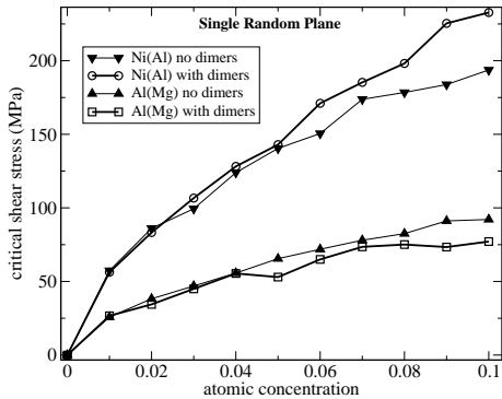
FIG. 15: Critical shear stress computed for Ni(Al) and Al(Mg) SRP solid solutions, within the elastic line model (ELM), as detailed in the text and sketched out in Fig. 6. The open symbols correspond to the same ELM as in Fig. 3. The full symbols correspond to the computations from an ELM where the solute atom dimers are approximated as the linear superimposition of the single solute atoms taking part to the dimers.
