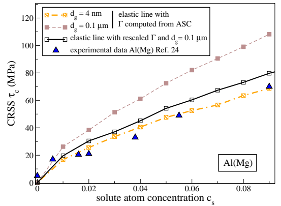
FIG. 17: ELM computations for the CRSS against solute atomic concentration c_s in Al(Mg), for different glide distances d_g (see legend). For comparison, the experimental data from Ref. [24] for Al(Mg) were reported as triangles. The rescaling for the line tension \Gamma is detailed in the text.
