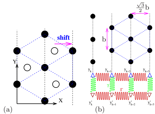
FIG. 6: (a) Schematic representation of the transformation from the fcc crystal sites to a perfect hexagonal lattice. (b) Schematic representation for the one-dimensional ELM with two bound elastic lines. Circles represent the lattice sites and the triangles correspond to the nodes of a discrete elastic lines. b stands for the norm of the Burgers vector (see Sec. II).
