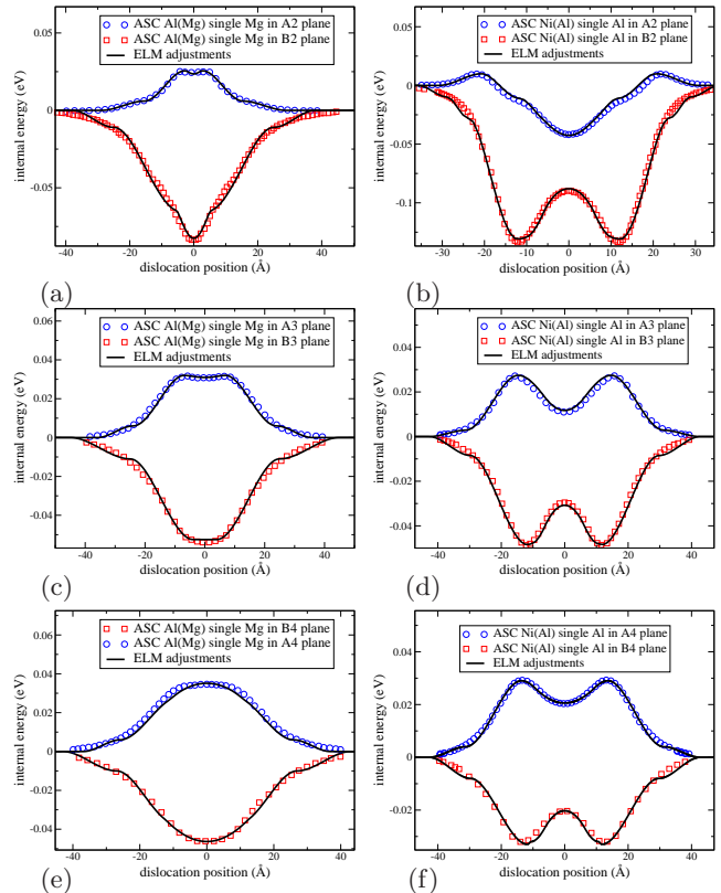
FIG. 10: (color online) Internal energy of the simulation cell U_{\text{cell}} for an edge dislocation bypassing a type I obstacle situated in the nearest planes (1\bar{1}1) above and below the glide plane. The planes are referred as a function of their apical height (see the text). The continuous lines have been obtained from the elastic ladder model (ELM), detailed in the text.
