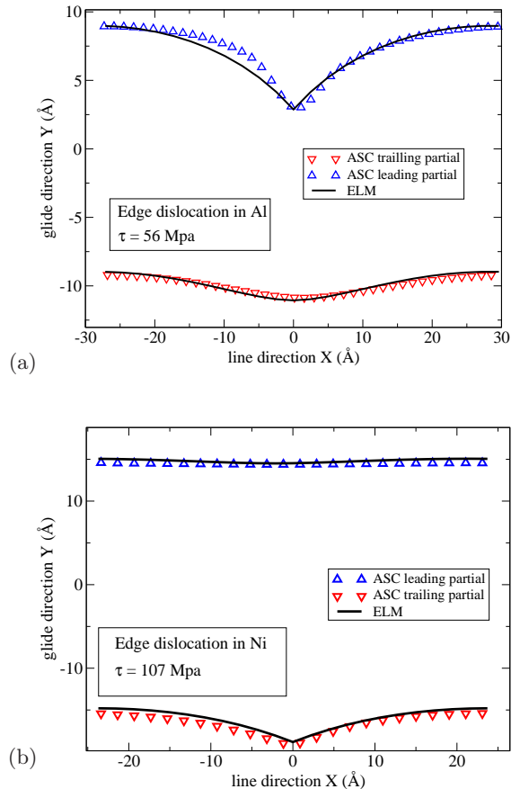
FIG. 7: Configuration for an edge dislocation, anchored on an arbitrary strong obstacle situated either in front of the trailing partial (a) or in between both partials (b), in a crystal of Al (a) and in a crystal of Ni (b) for different applied shear stresses (see insets). The triangles represent the dislocation segments computed within atomic-scale simulations and the continuous lines correspond to the results from the elastic line model presented in Figs. 6 (b).
