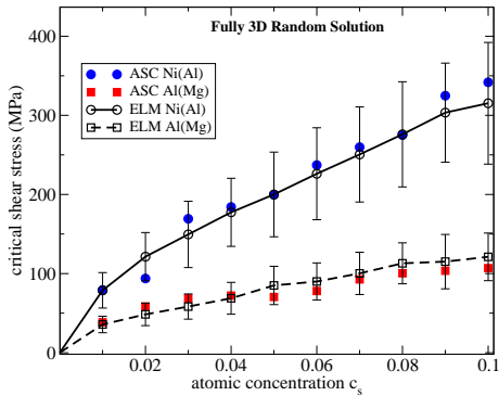
FIG. 5: Same as in Fig. 3 and Fig. 4 but for fully random solid solutions (referred in the text as to FRD). The corresponding elastic line model (ELM) is detailed in Sec. III.
