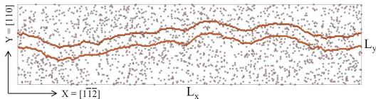
FIG. 1: (color online) Plane view for an edge dislocation pinned by Mg solute atoms in Al(Mg) alloy, modeled within EAM. 23 The Mg atoms situated in the nearest planes that bound the (1\bar{1}1) glide plane are colored in grey while the atoms involved in the Shockley partial dislocations are colored in orange. The rest of the crystal atoms are not shown. The Mg concentration is c_s = 2 at. %.
