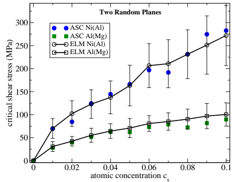
FIG. 4: Same as in Fig. 3 but for different constrained solutions, referred as to TRP in the text, made of a pure crystal with solute atoms situated in the two contiguous planes that bound the dislocation glide plane. The corresponding elastic line model (ELM) is detailed in Sec. III.
