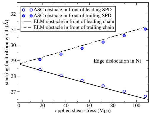
FIG. 8: Width of the stacking fault ribbon d_{\text{SPD}} for an edge dislocation anchored on an arbitrary strong obstacle situated either in front of the trailing partial or in between both partials, in a crystal of Al (a) and in a crystal of Ni (b). The symbols represent the computations from atomic-scale simulations and the lines correspond to the elastic line model presented in Figs. 6 (a-b) with the same geometric parameters given in Ref. [31].
