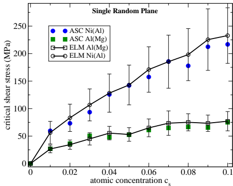
FIG. 3: Critical resolved shear stress computed for Ni(Al) and Al(Mg) from the atomic-scale computation (ASC) (full symbols) for an edge dislocation passing through a crystal with a single (1\bar{1}1) random plane situated just above the glide plane (referred as SRP in the text). The elastic line model (ELM) predictions (open symbols with full lines) were obtained as detailed in Sec. III. The error bars corresponds to the mean square root of the ELM sampling.
