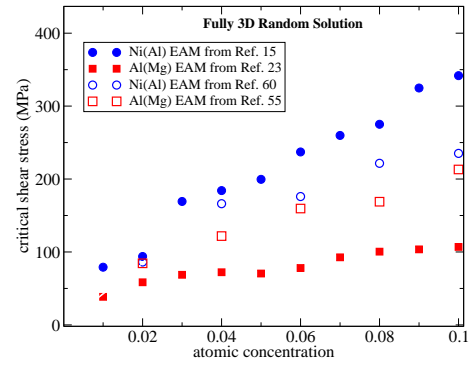
FIG. 19: Critical resolved shear stress computed from ASC for the fully random solid solutions of Al(Mg) and Ni(Al) with different concentrations c_s and with the geometry given in Ref. [31]. Different EAM are employed for the two systems (see legend). The EAM chosen for the present study are those developed by Liu et al. 23 for Al(Mg) and by Rodary et al. 15 for Ni(Al).
