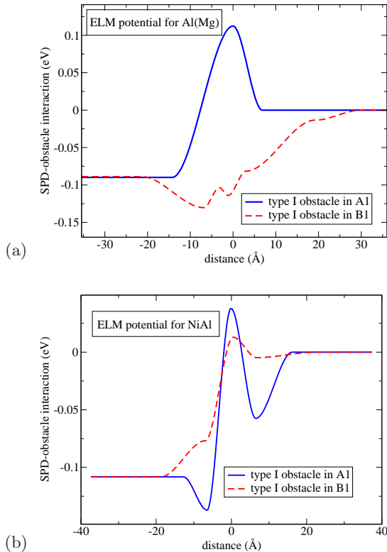
FIG. 9: Interaction potentials V_{I-j} between the elastic line corresponding to the leading partial, for different systems and different positions of the obstacle above ( A1 ) and below ( B1 ) the glide plane. These potentials have been constructed with a series of cubic polynomials, interpolating the coordinates for the first derivative zeroes.
