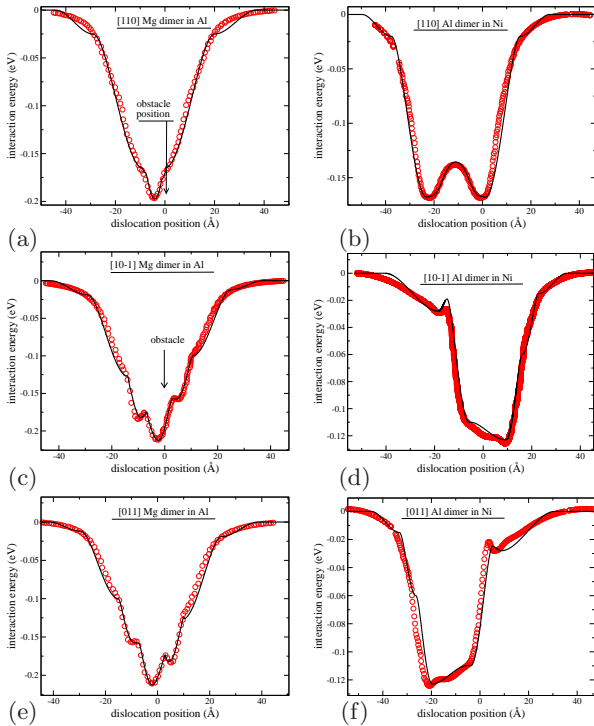
FIG. 13: Same as in Figs. 12 (a-f) but for dimers situated in (\bar{1}\bar{1}1) planes just below the glide plane j = (B1) .
