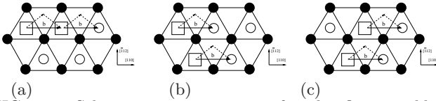
FIG. 11: Schematic representation for the first neighbor dimer configurations in the (1\bar{1}1) plane. Portion of the 2 nearest (1\bar{1}1) planes that bound the dislocation glide plane. The square symbols correspond to the solute atoms whereas the circles represent crystal atoms. Open symbols represent atoms situated above the glide plane, the full symbols the ones below the glide plane. The arrows indicate the relative motion of the atom in the course of the dislocation passage.
