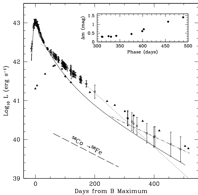
FIG. 18.—Comparison between the UVOIR bolometric light curve of SN 1998bw and the hypernova model by Iwamoto et al. (1998; solid line ). The dotted line represents an extrapolation of a least-squares fit to the data in the range 50–200 days, while the dot-dashed line is a fit to the data in the phase range 376–490 days. The dashed line corresponds to the ^{56}\text{Co} \rightarrow ^{56}\text{Fe} decay rate, expected for full \gamma -ray trapping. The plot in the upper right part of the figure shows the deviations of the observed data from the extrapolation on the early light curve (50–200 days; see text). For comparison, the bolometric light curve of SN 1987A (Bouchet, Danziger, & Lucy 1991) is also plotted ( filled triangles ).
