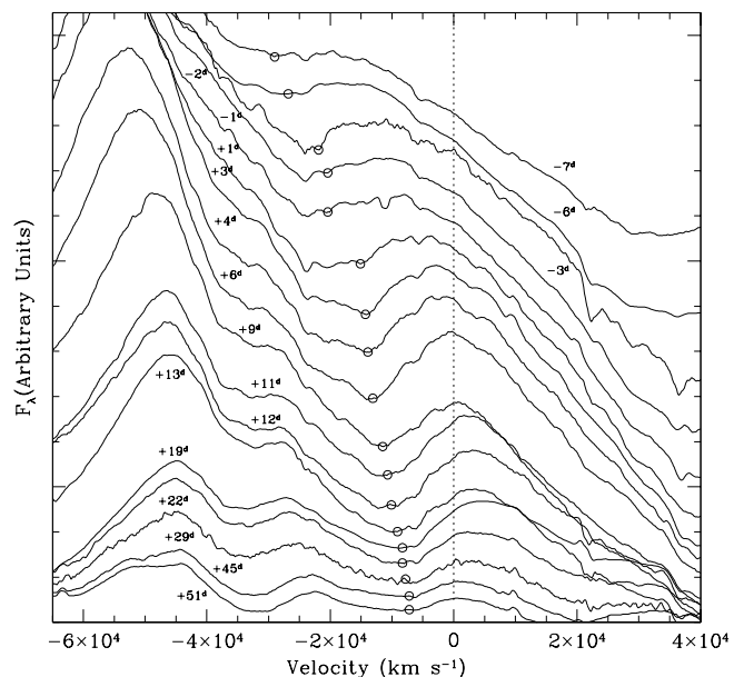
FIG. 4.—Evolution of the \text{Si II } \lambda 6355 region. The empty circles mark the value that has been assumed to represent the photospheric velocity.
