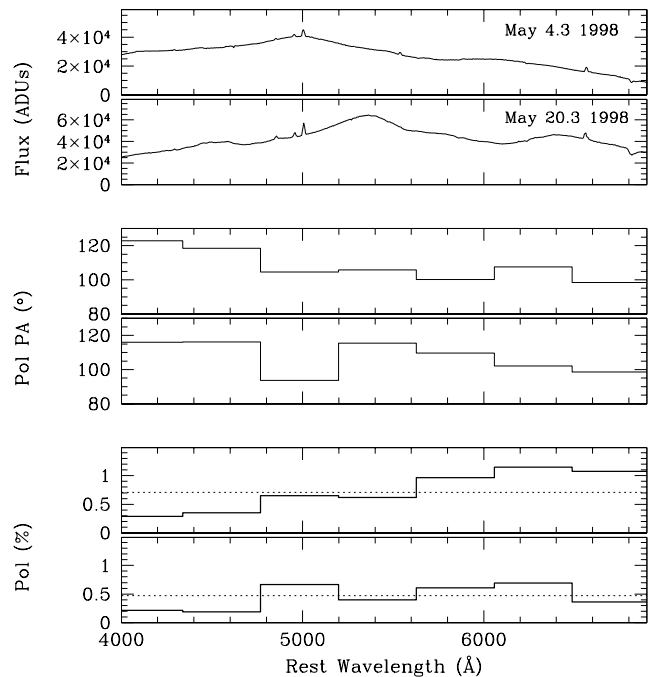
FIG. 6.—Raw spectrum (ADU), position angle (degrees) and linear polarization degree (percent) are shown from the EFOSC2 spectro-polarimetry observations at day -7 (upper panel) and day +10 (lower panel). Wavelengths are corrected to the host galaxy rest frame ( v_{\text{gal}} = 2532 \text{ km s}^{-1} ; see § 5). The linear polarization and position angle data have been binned into 200 channel increments to increase the signal-to-noise ratio.
