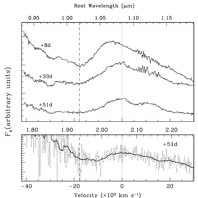
FIG. 8.—Upper panel: IR spectroscopic evolution of SN 1998bw from day +8 to day +51 in the region of He I 1.083 \mu\text{m} . The vertical dashed line marks the expansion velocity measured for He I 1.083 \mu\text{m} on day +8. Lower panel: Region of He I 2.058 \mu\text{m} at day +51. The solid line is a smoothed version of the spectrum. A 350 \text{ \AA} -wide boxcar filter was used.
