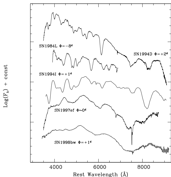
FIG. 3.—Comparison between SN 1998bw and other SNe at maximum light. Data are from Patat et al. (1996; 1994D), Harkness et al. (1987; 1984L), ESO-KP database (1994I), and Garnavich et al. (2001, in preparation; 1997ef). All spectra have been corrected to the parent galaxy rest frame adopting the following recession velocities: SN 1998bw, 2532 \text{ km s}^{-1} (see § 5); SN 1997ef, 3504 \text{ km s}^{-1} ; SN 1994I, 463 \text{ km s}^{-1} ; SN 1994D, 448 \text{ km s}^{-1} ; SN 1984L, 1934 \text{ km s}^{-1} (de Vaucouleurs et al. 1991).
