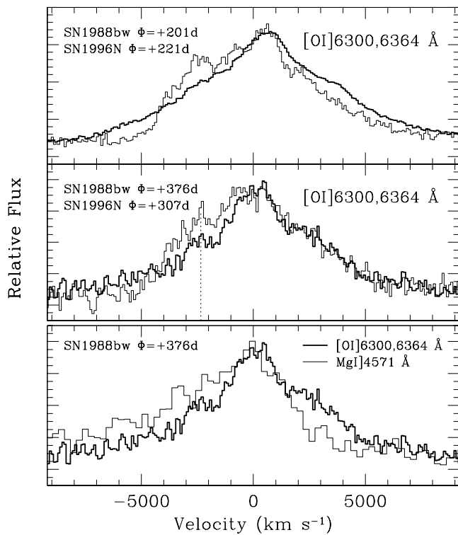
FIG. 12.— Upper and middle panels: The [O I] \lambda\lambda 6300, 6364 line profile at two different epochs for SN 1988bw ( thick line ) and SN 1996N ( thin line ; Sollerman et al. 1998). The vertical dotted line is placed at the position of the unidentified feature (see text). Velocities are computed from the \lambda 6300 doublet component. Lower panel: Comparison between the profiles of [O I] \lambda\lambda 6300, 6364 ( thick line ) and Mg I \lambda 4571 ( thin line ) for SN 1988bw at +376 days.
