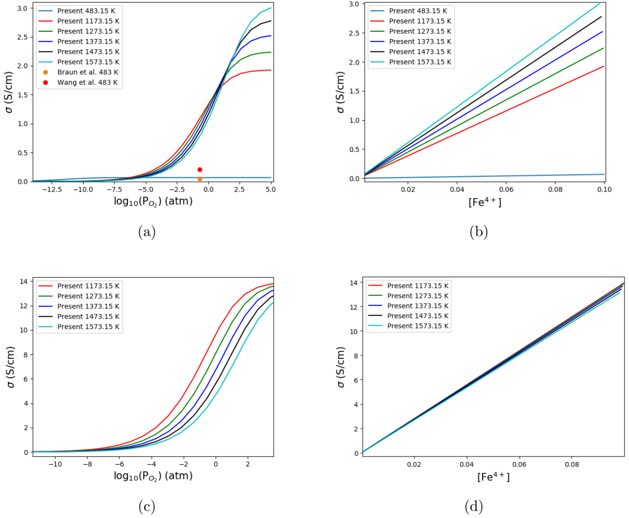
FIG. 15: Hole conductivity as a function of partial oxygen pressure and as a function of hole concentration. (a), (b): E_c = 0.3 eV. (c), (d): E_c = 0.1 eV.
