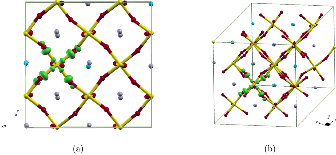
FIG. 7: Isosurfaces (20 % of the maximal value) of the probability amplitude of the wave-functions associated to the hole states in LSF for (a) x \approx 0.1 and (b) x \approx 0.6 .
