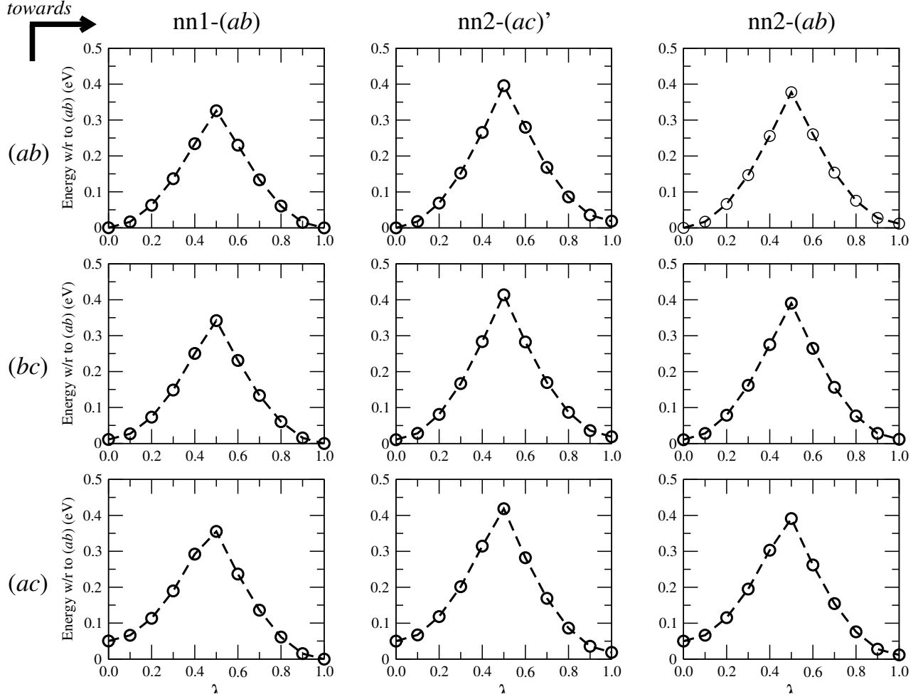
FIG. 5: Energy profile for nine hopping paths of the self-trapped hole polaron, from (ab) , (bc) , and (ac) onto two nearest-neighbor sites called nn1 and nn2 , associated with three states of the polaron, see Fig. 3.
