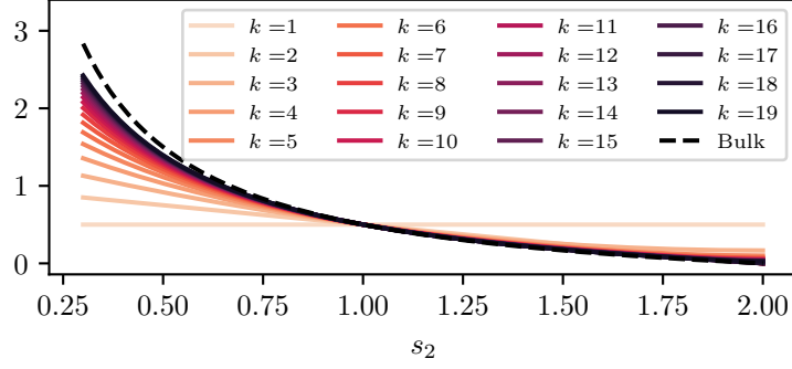
Figure 6: Plot of the polynomial 1/2 + \sum_{\ell=1}^{n-1} (1 - \ell/n)(1 - s_2)^\ell appearing in (46) for different n compared to 1/s_2 - 1/2 (bulk).
