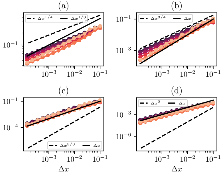
Figure 3: L^2 errors at the final time for two forward centered initialisations (38) (top) and (39) (bottom). Since the letter irremediably perturbs the conserved moment feeding the bulk Finite Difference scheme, the orders of convergence above one are lowered. Color legend for the relaxation parameter s_2 : ● for s_2 = 1.1 , ● for s_2 = 1.2 , ● for s_2 = 1.4 , ● for s_2 = 1.6 , ● for s_2 = 1.8 , and ● for s_2 = 2 .
